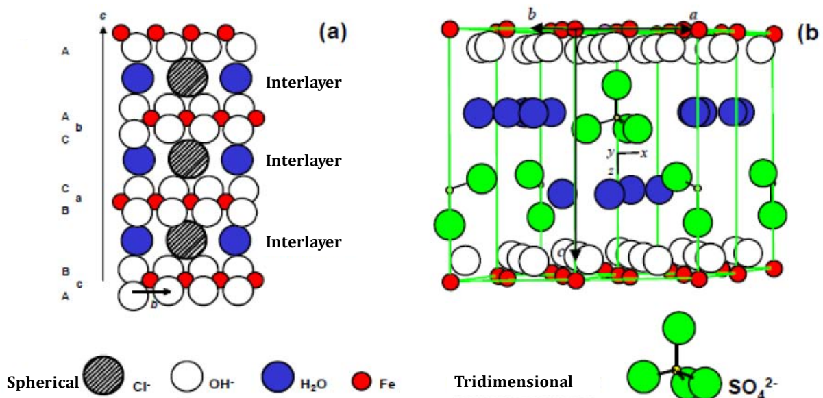
Figure 2: Structure of green rusts: (a) GR1 (Cl) (b) GR2 (SO 4 ) (Refait et al. , 1998; Simon et al. , 2003). This material was reproduced with the permission of Elsevier.
