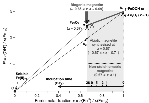
FIGURE 4. \text{Fe}^{2+} - \text{Fe}^{3+} mass-balance diagram showing the composition domain of biotic and abiotic magnetite and the ferric molar fraction x of the suspension at different incubation time (right bottom).
