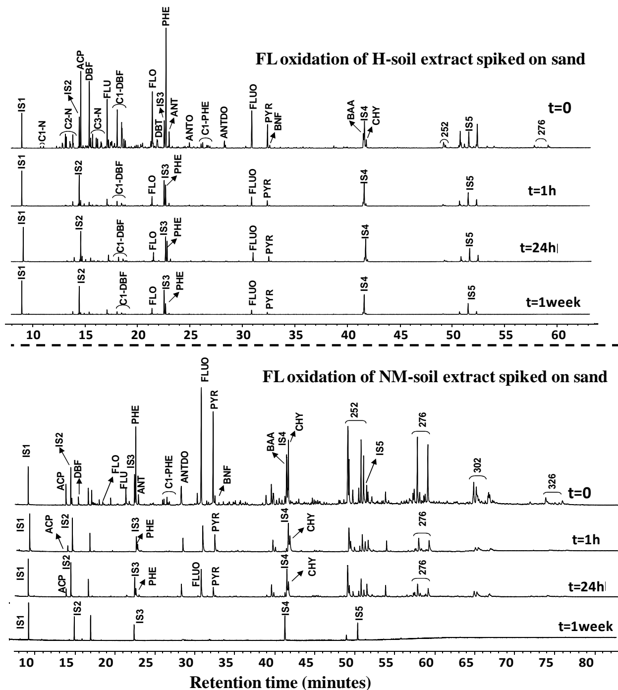
Figure 4: Molecular distribution obtained by GC-MS of H and NM organic extract (spiked on sand) before oxidation ( t=0 ) and after different oxidation times by FL oxidation ( H_2O_2 + magnetite). The compounds are detailed in Table S1. Experimental conditions were: solid matrix=2g, Volume of solution=20mL. Oxidant dose was used according to H_2O_2:Fe molar ratio of 20:1.
