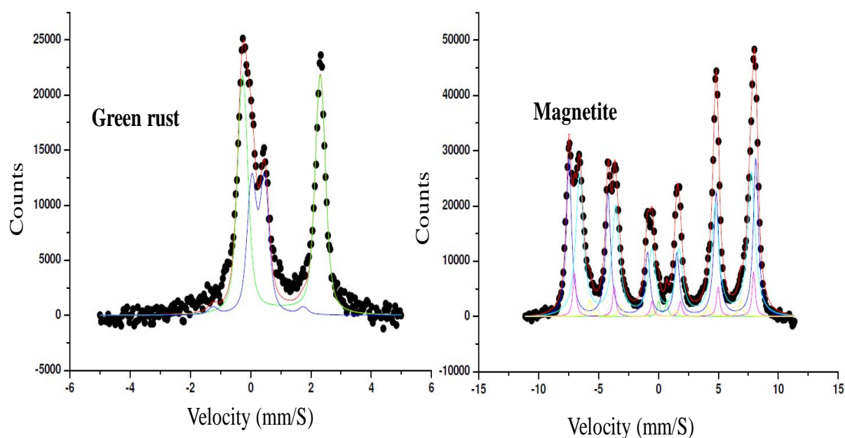
Figure 1. Mössbauer spectra of GR (A) and magnetite (B) generated through Fe II reaction with Ferrihydrite.
