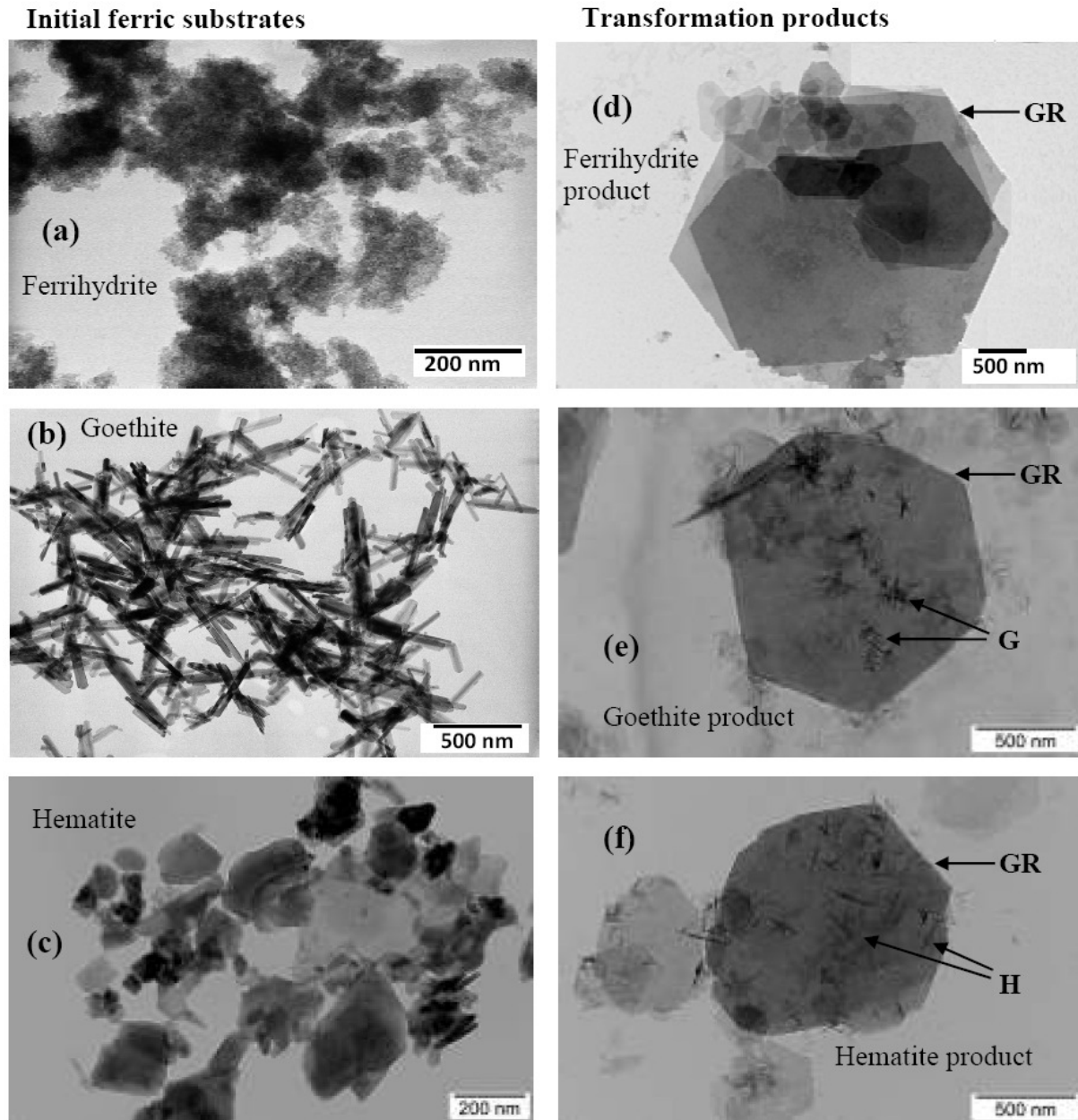
Figure 2: TEM images of initial ferric substrates (a: ferrihydrate, b: goethite and c: hematite) and their transformation products (d: ferrihydrate product, e: goethite product and f: hematite product).
