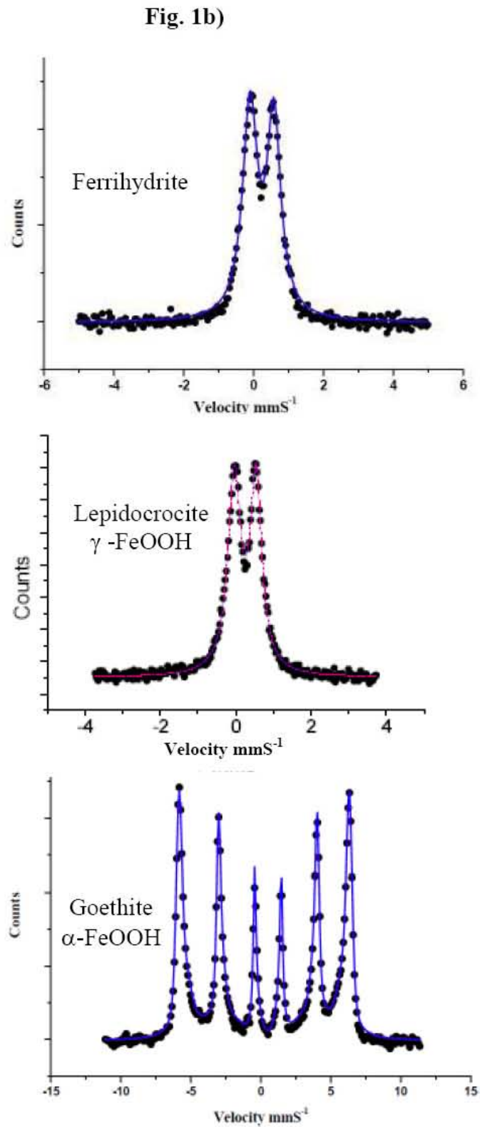
Figure 1: XRD diffractograms (a) and Mössbauer spectra (b) of original ferric substrates, ferrihydrite (F), goethite (G1) and lepidocrocite (L)
