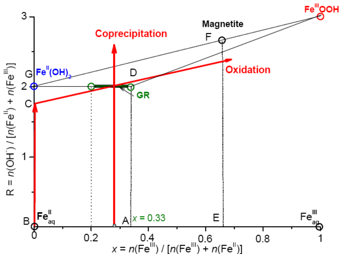
Figure 4: \text{Fe}^{\text{II}} - \text{Fe}^{\text{III}} mass-balance diagram showing the co-precipitation and oxidation [Adapted from Fig. 1 of (Ruby et al. , 2006a; Ruby et al. , 2010)]
