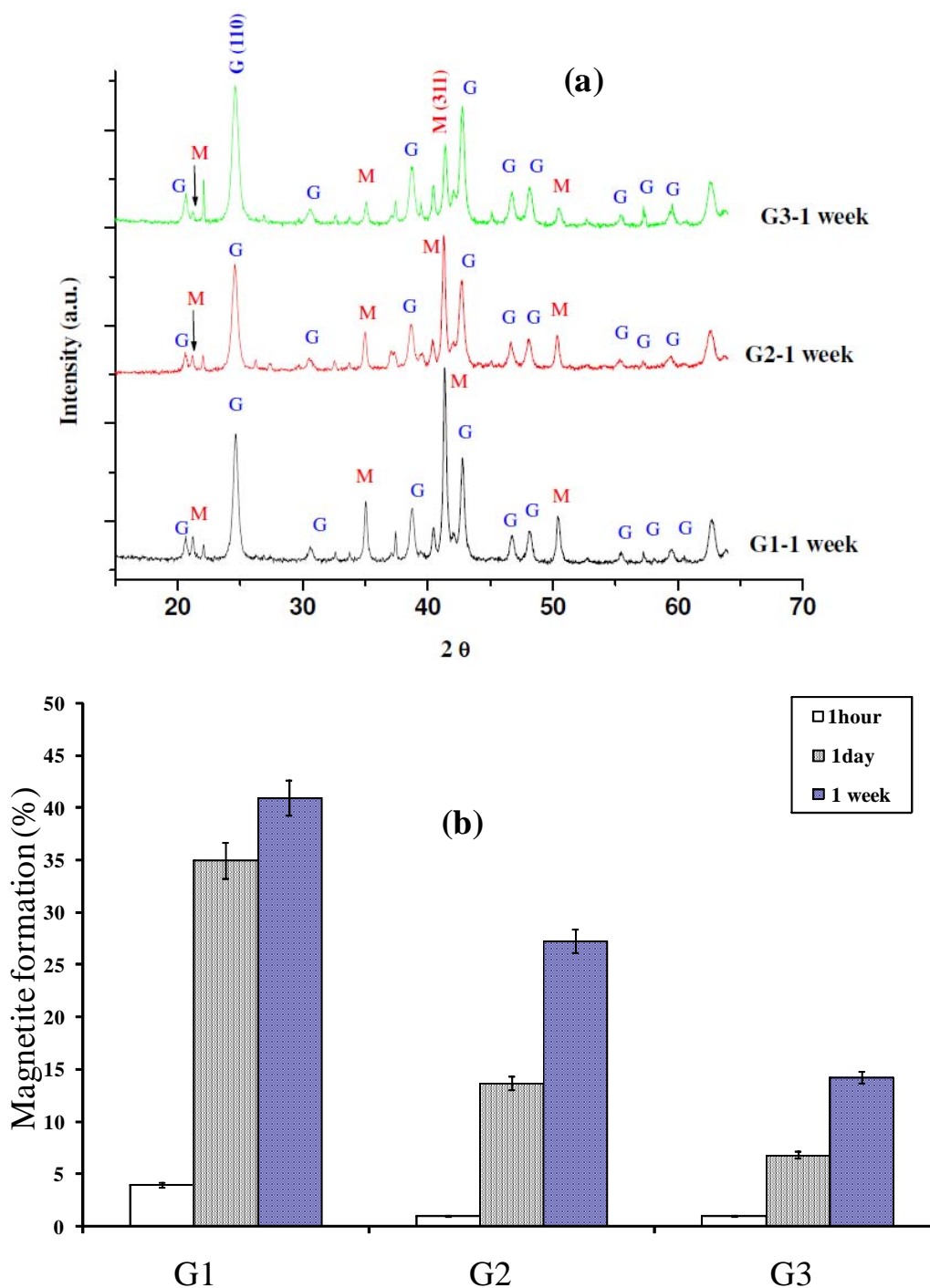
Figure 6: (a) XRD diffractograms of the transformation products of three kinds of goethite (G1, G2 and G3), obtained after aging time of 1 week and (b) the histogram comparing the magnetite formed (%) from three goethites after aging time of 1 hour, 1 day and 1 week.
