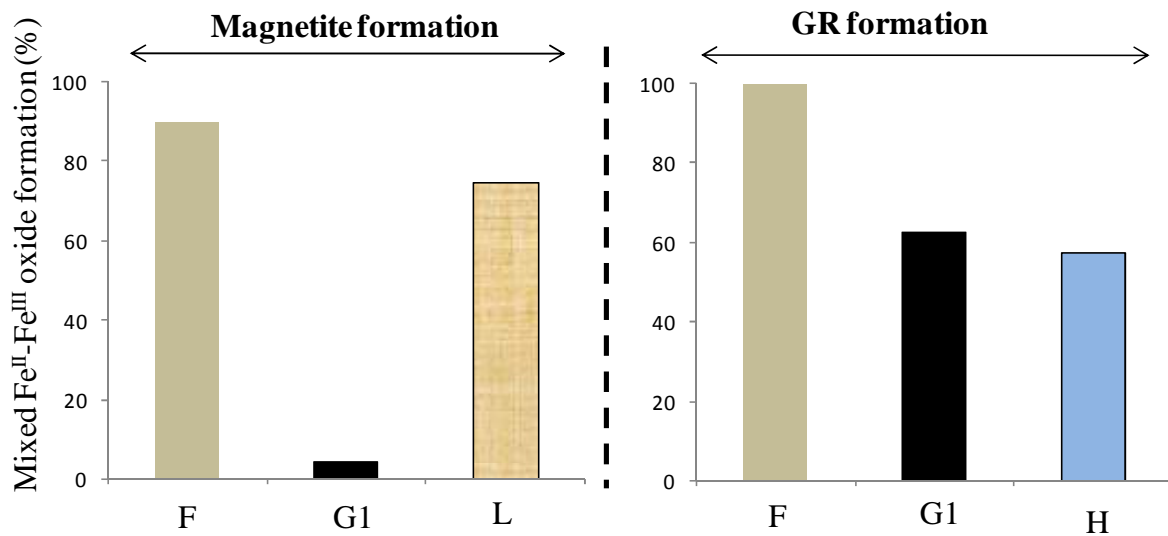
Figure 1.2: Formation extent of magnetite or GR after aging time of one hour from ferrihydrite (■), goethite (■), lepidocrocite (■) and hematite (■). It is represented in % and based on the measurements by Mössbauer spectroscopy. (* Lepidocrocite and hematite are transformed only into magnetite or GR respectively.)
