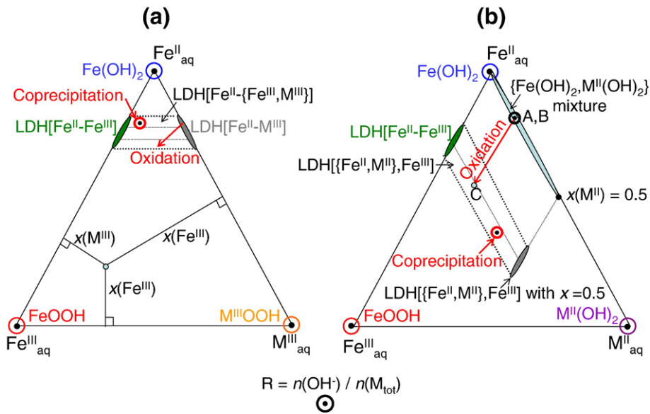
Fig. 2. Ternary mass-balance diagrams showing the domains and syntheses routes of \text{M}^{\text{III}} (a) and \text{M}^{\text{II}} (b) substituted iron-based LDHs.
