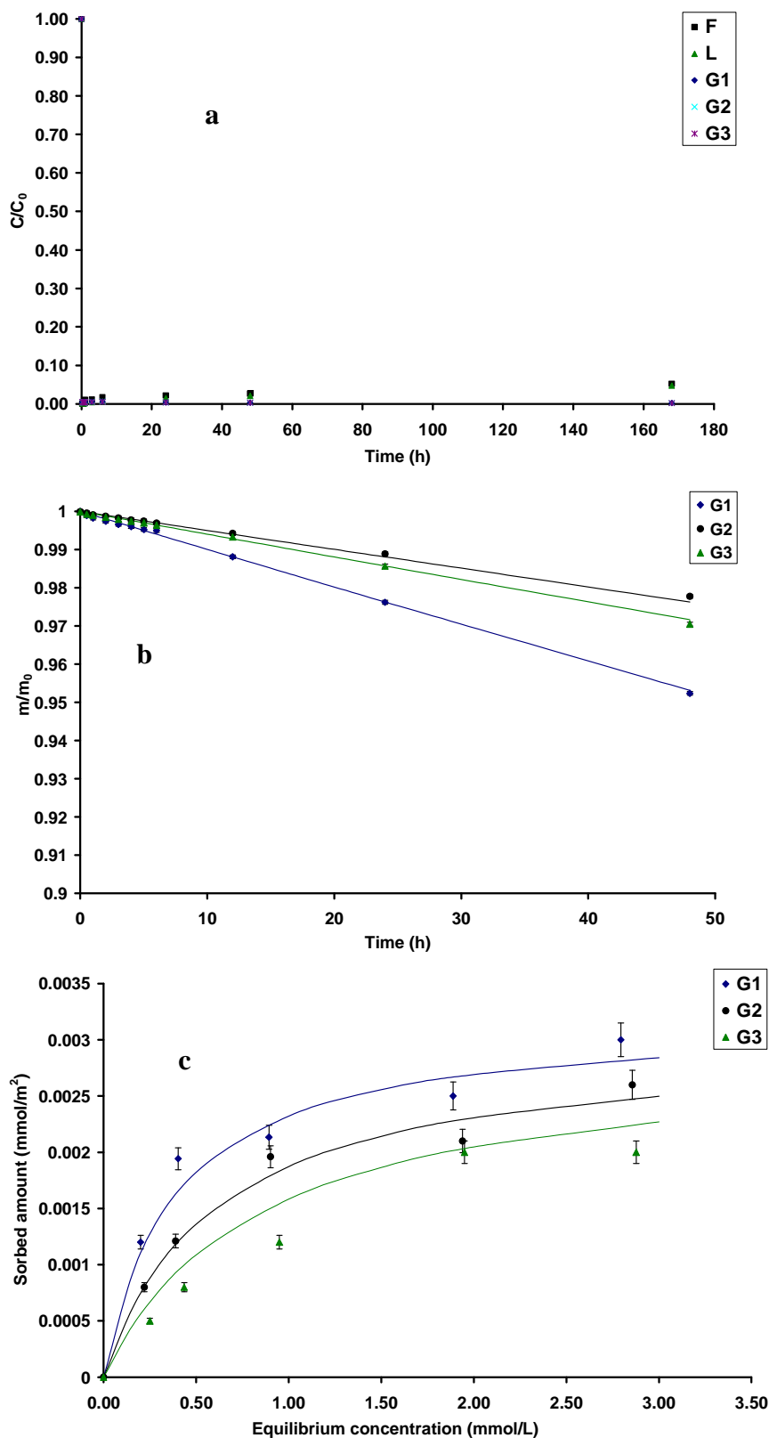
Figure 7: (a) Relative concentration ( C/C_0 ) of aqueous Fe(II) during the transformation reaction. Input concentration C_0=50 mM, the pH values are reported in Table 1. (b) Reductive dissolution rate of three goethites at pH3. m/m_0 is the fraction of undissolved iron oxide. [ascorbic acid] =10 mM, [solid] = 50 \text{m}^2/\text{L} ;
