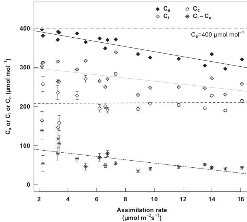
Figure 5: During the PPFD experiment, variations of CO 2 mole fraction in the atmosphere ( C_a , black diamonds and black continuous line), intercellular airspace ( C_i , grey diamonds and grey continuous line) and chloroplast ( C_c , empty diamonds and black dashed line) versus assimilation rate ( A ). Each point is mean (30~40 single measurements), error bar are standard deviation.
