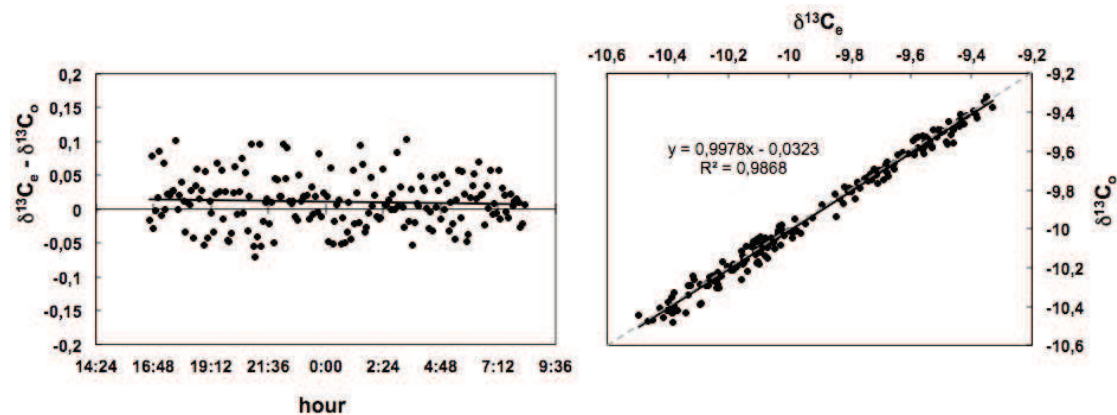
Figure A6: On the left panel, recorded difference between \delta^{13}C_e - \delta^{13}C_o (isotopic composition of air entering and leaving the photosynthesis chamber) with an empty chamber during 15h. On the right panel, the corresponding correlation between \delta^{13}C_e and \delta^{13}C_o , the grey dashed line represent the 1:1 relationship. The variation of \delta^{13}C_e (from -9.3‰ to -10.6‰) was due to changes in the atmospheric \delta^{13}C at the Université de Nancy on Julian day 112, 2009.
