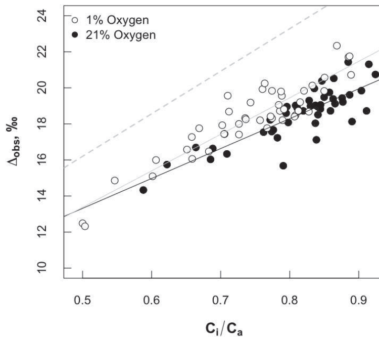
Figure 2: Variations of observed discrimination against 13 CO 2 ( \Delta_{\text{obs}} , ‰) with the ratio of intercellular/atmospheric mole fraction ( C_i/C_a ) ratio under 21 (black points) and 1 % O 2 (white points) in three Eucalypt species. Each point is the mean of three measurements at 180s intervals. The dotted line represents the discrimination computed from the simple form of Farquhar's model ( \Delta_i , Eq.1).
