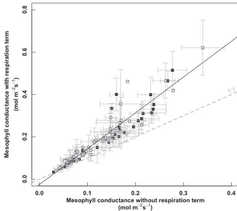
Figure 6: Mesophyll conductance g_m as computed by taking into account the contribution of respiration and photorespiration to ^{13}\text{CO}_2 discrimination vs without taking them into account (i.e., fractionation factors e and f set to 0 in Eqn. 7). Results obtained under changing \text{CO}_2 (black squares) or irradiance (white squares). The dashed line represents
