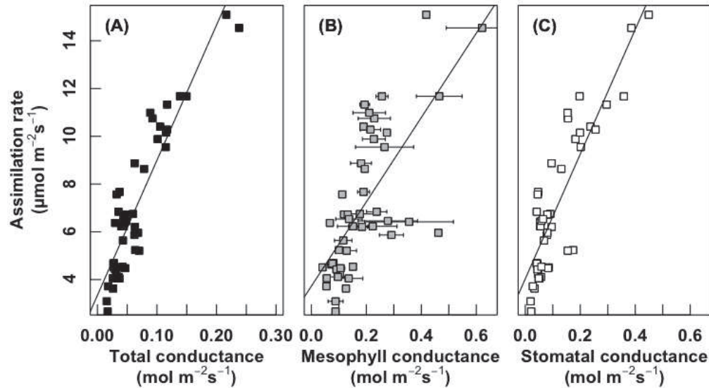
Figure 5: Relationships between net CO 2 assimilation rate ( A ) and (A) total leaf conductance to CO 2 ( g_t , black squares), (B) internal conductance to CO 2 ( g_m , grey squares) and (C) stomatal conductance to CO 2 ( g_s , white squares) under varying PPFD.
