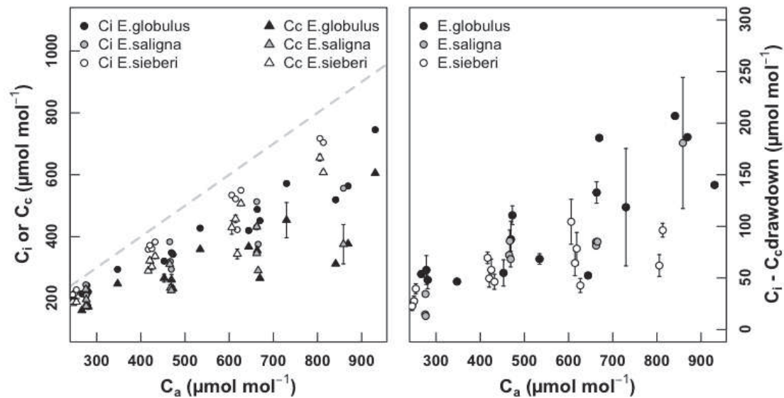
Figure 3: Left: CO 2 mole fraction in the substomatal cavities ( C_i , disks) and at carboxylation sites ( C_c , triangles) as a function of C_a . The dashed grey line is the 1:1 relationship. Right: C_i - C_c drawdown as a function of C_a . Each point represents the mean of 1-3 analytical measurement mean \pm SE, with E. globulus in black, E. saligna in grey, and E. sieberi in white.
