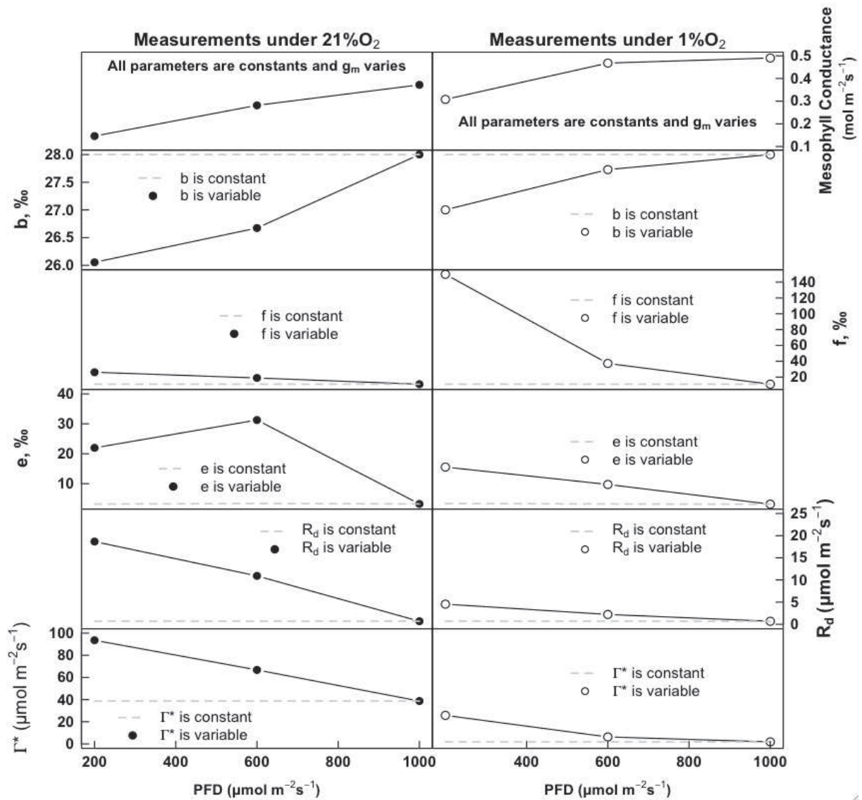
Figure 7: We tested the hypothesis of a stable g_m and calculated the variations of each parameter needed to obtain the same \Delta^{13}\text{C} as observed with a constant g_m across irradiance variations, for each parameter (from the top to the bottom: b , f , e , R_d and \Gamma^* ). Left panels (filled circles) indicate measurement under 21% O 2 and right panels (empty circles) indicate measurement under 1% O 2 . Data were recorded on Eucalyptus sieberii (unpublished). g_m was calculated with the isotopic method from measurements performed with a calibrated TDLAS, using the standard parameterization described in Table 3, except \Gamma^*=38.7 and 1.85 \mu\text{mol mol}^{-1} under 21% and 1% O 2 , respectively. Each point is an average of three measurements taken at 180s intervals.
