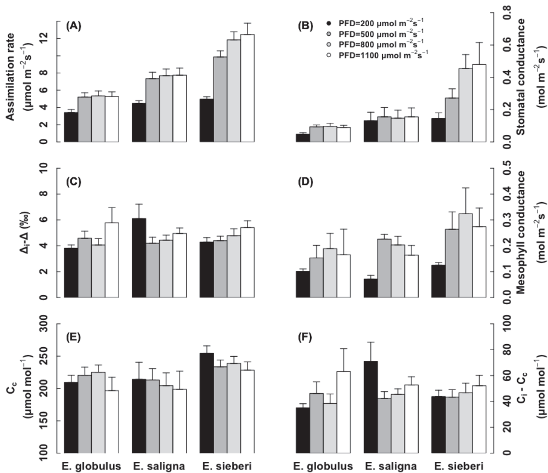
Figure 4. (A) Net \text{CO}_2 assimilation rate ( A ), (B) stomatal conductance to water vapour ( g_s ), (C) difference between predicted and measured isotopic discrimination ( D_i - D ), (D) mesophyll conductance
