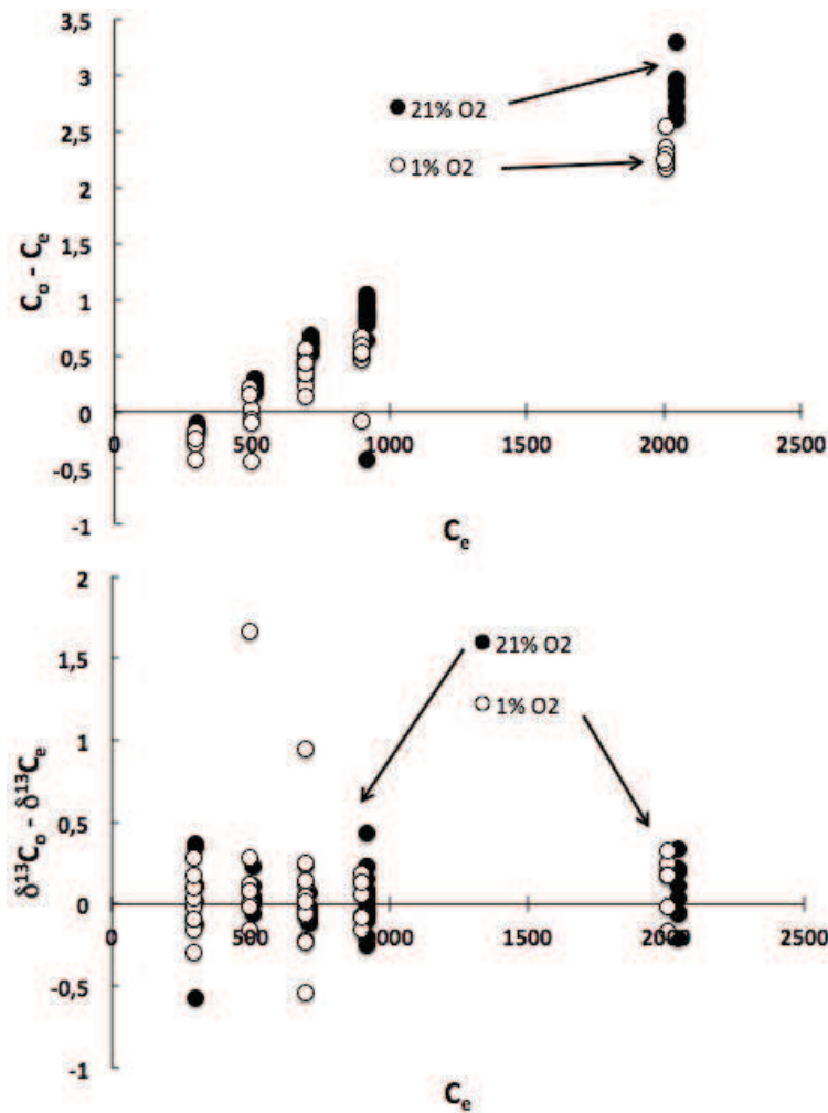
Figure A2: Upper panel: Difference between CO 2 molar fraction entering and leaving the photosynthesis chamber ( C_e and C_{e0} , respectively in \mu\text{mol mol}^{-1} ) versus CO 2 mole fraction entering the chamber ( C_e ). Measurements were performed under 21 (black dots) and 1% O 2 (empty circles).
