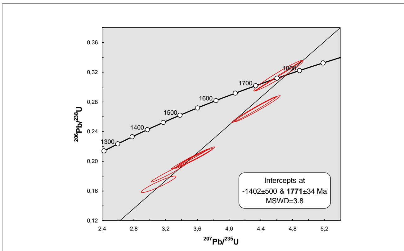
Figure 3.30. The \text{Pb}^{206}/\text{U}^{238} vs \text{Pb}^{207}/\text{U}^{235} concordia diagram for the uraninite from the Cheptjavr ore-showing [sample 56-3] (by SIMS CAMECA IMS-3F - CRPG-CNRS, Nancy, France).
