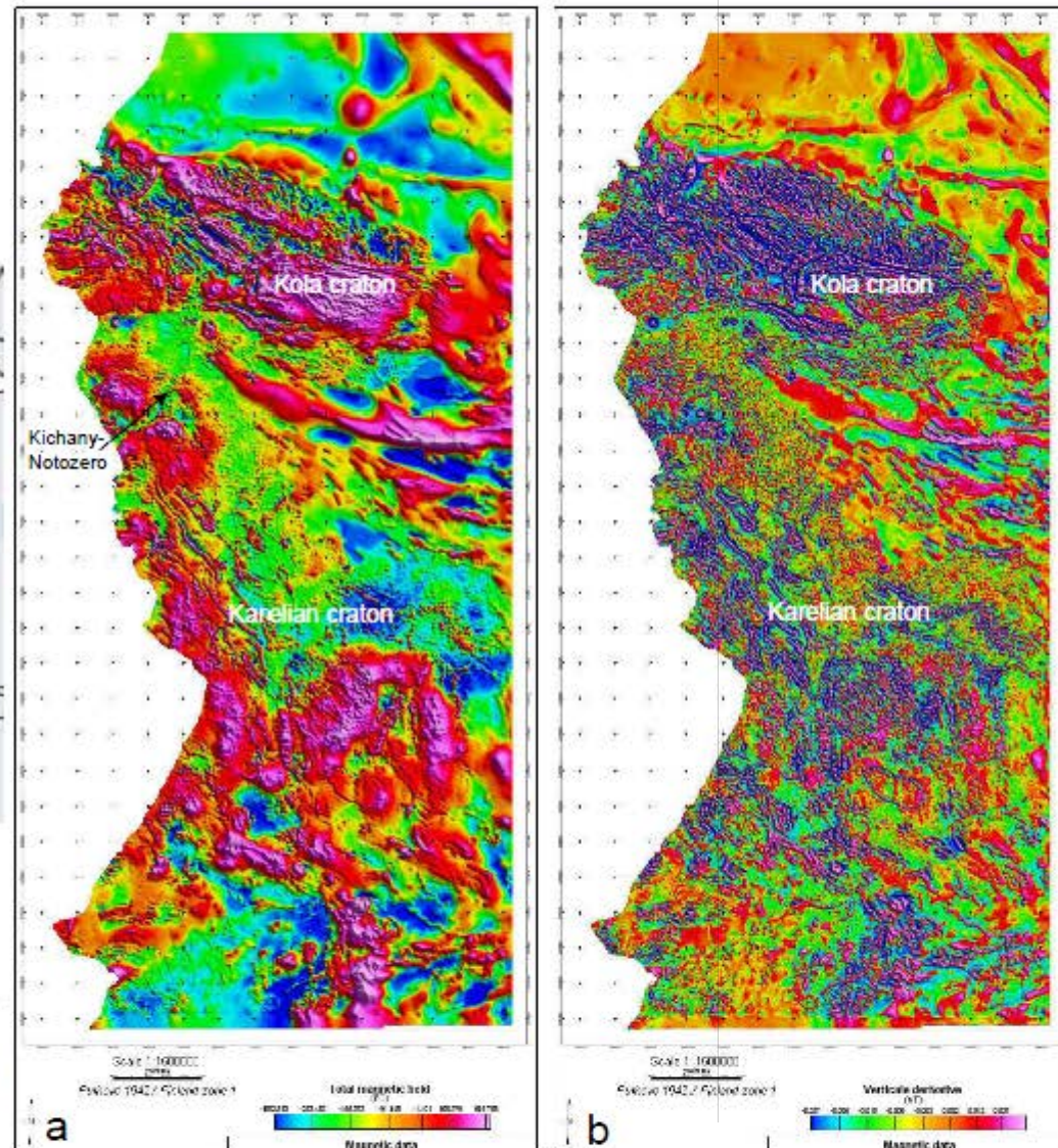
Figure 1.15. Aeromagnetic maps of the Karelian craton and Lapland-Kola orogen a: Total Magnetic field; b: First vertical derivative of the total Magnetic field
