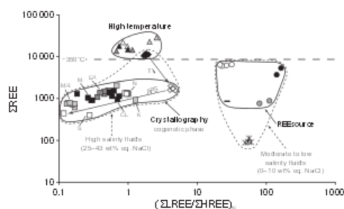
Fig. 4 Rare earth element abundance ( \Sigma\text{REE} ) vs. REE fractionation ( (\Sigma\text{REE}/\Sigma\text{HREE})_0 ) for analyses presented in Fig. 2 (same symbols used in both figures). REE and (\Sigma\text{REE}/\Sigma\text{HREE})_0 values are shown in Table 2 (Electronic Supplementary Material). The main parameters controlling REE content in the uranium oxides for each deposit type are highlighted (bold italic name and black line). REE abundance in hydrothermal deposit reflects the salinity of the ore fluid (small dashed lines). No REE fractionation ( \Sigma\text{REE}/\Sigma\text{HREE} = 1 ) is seen in deposits which formed at T > 350^\circ\text{C} (big dashed line). Below this temperature, the crystallography of uranium oxides is a key parameter. For synmetamorphic and unconformity-related deposits, the REE contents are also dependent of the crystallisation of co-genetic phase (APS). For vein-type and roll-front deposits, the REE source controls the REE pattern (see text for explanation). S.: Sue, M.R.: McArthur River, M.: Millennium, E.P.: Eagle Point, N.: Nabarlek, K.: Koongarra, C.L.: Cigar Lake.
