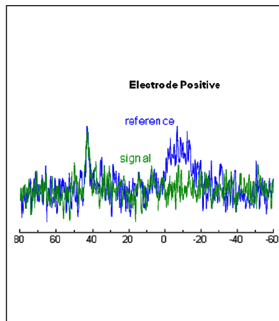
Figure III-30 : RMN REDOR \{^{19}\text{F}\}^{27}\text{Al}
