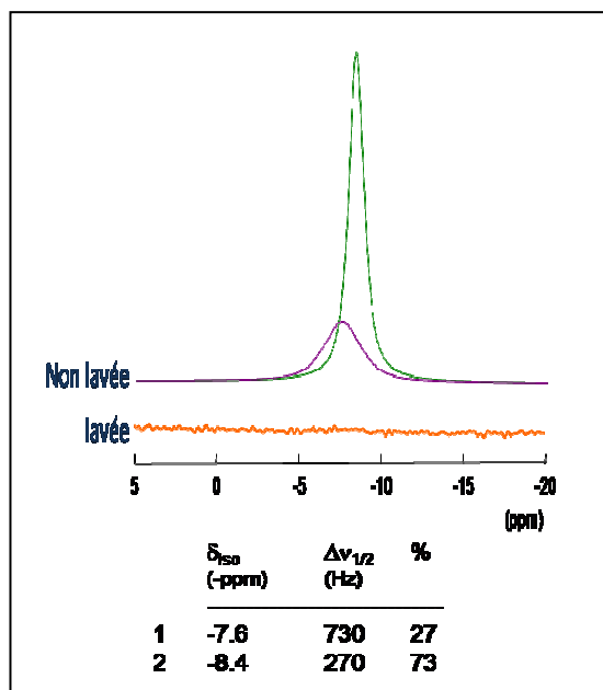
Figure III-29 : RMN MAS ^{11}\text{B}
