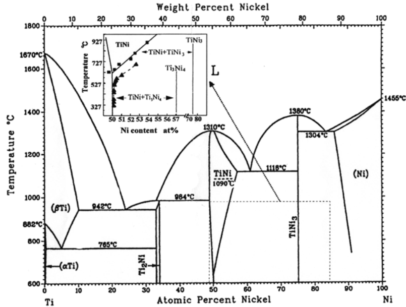
FIGURE A.1 – Diagramme de phase de l'alliage Nickel-Titane Massalski, ASM International and Materials
