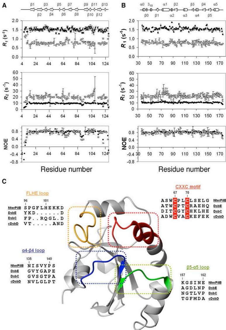
Figure 3. ^{15}\text{N} Relaxation Parameters of the Mixed Disulfide Complex nDsbD-SS-NterPilB and Interaction Areas on the Trx-like Partner of nDsbD
