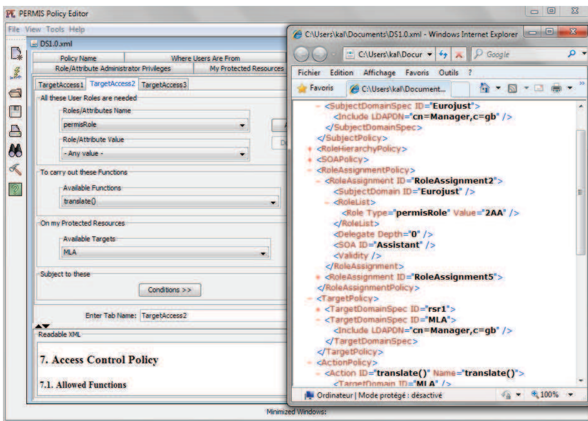
Figure 6.12: Policy editor for DS1
