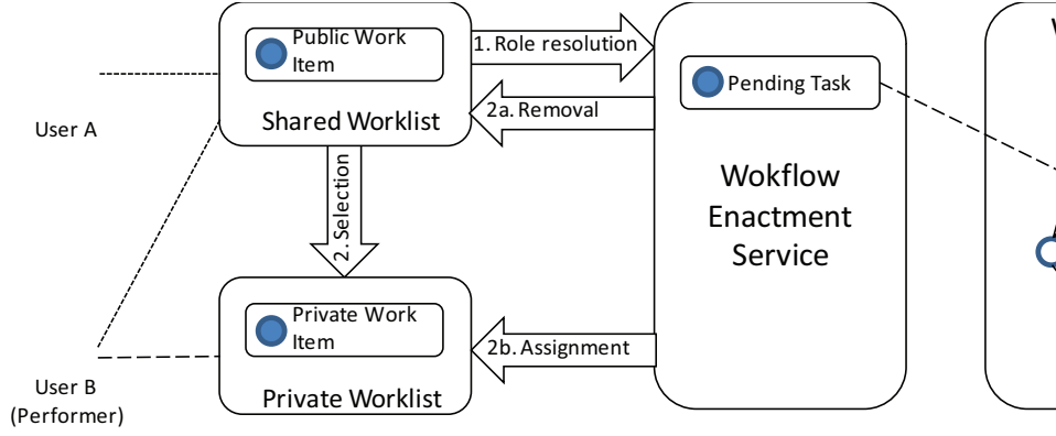
Figure 2.3: Role resolution procedure at runtime
