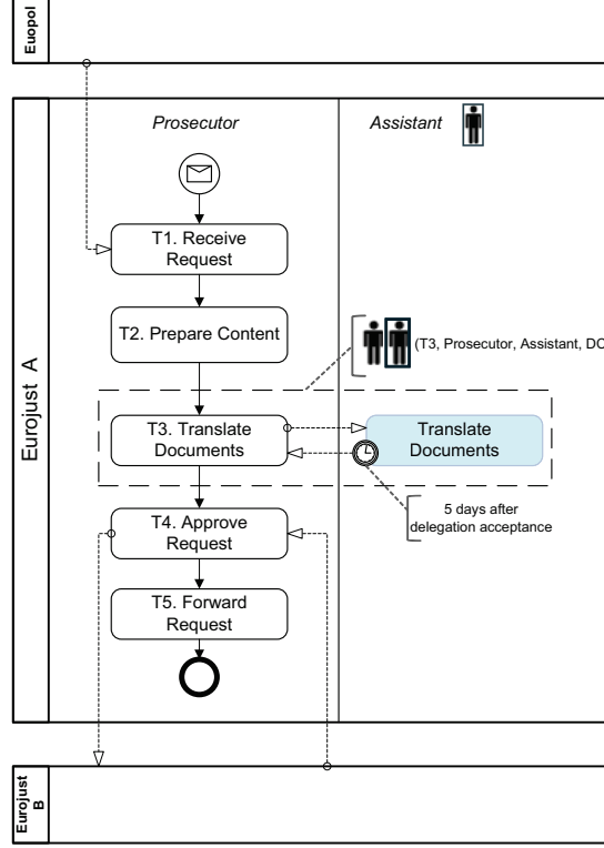
Figure 5.1: Local delegation scenario from the MLA example
