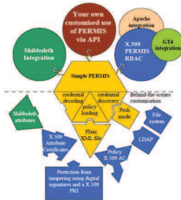
Figure 6.9: PERMIS decision engine architecture
