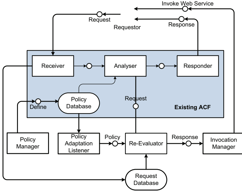
Figure 5.6: Architectural extensions supporting delegation policies
