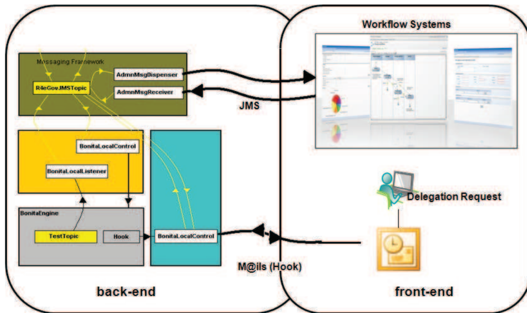
Figure 6.4: Integrating the Bonita engine within the core R4eGov framework
