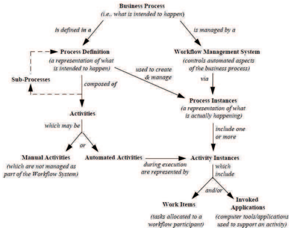
Figure 3.1: Workflow terminology
