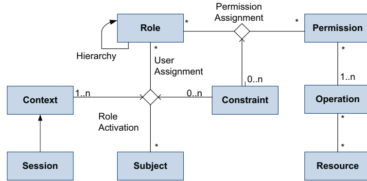
Figure 3.9: RBAC Sessions
