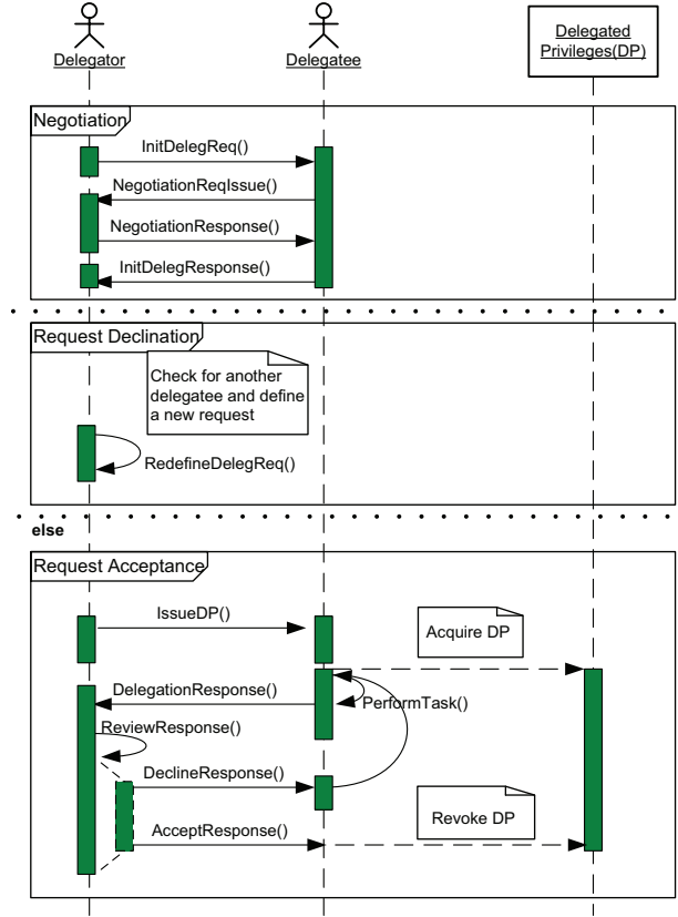
Figure 4.7: Delegation protocol negotiation-based
