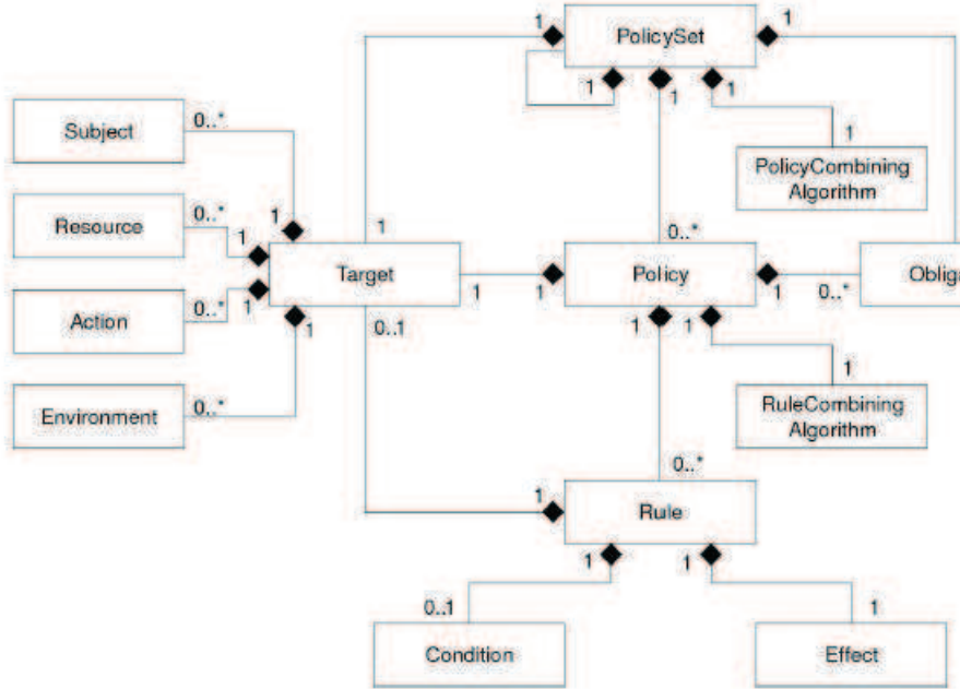
Figure 3.11: XACML policy language model
