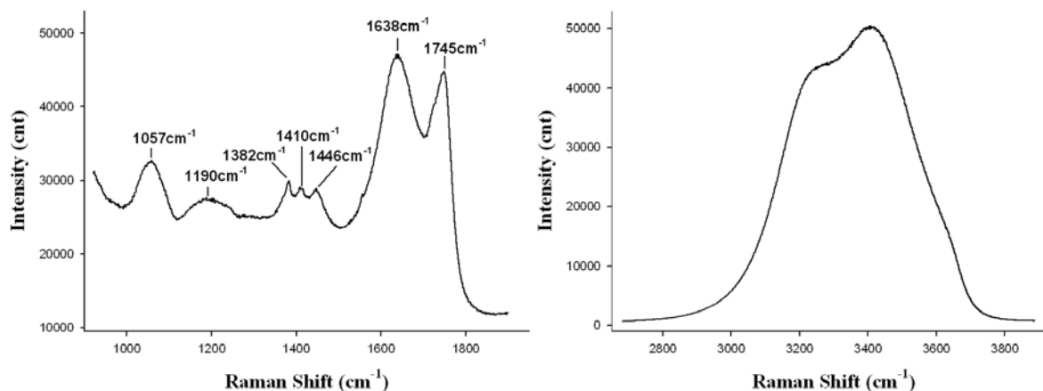
Figure II-29 The Raman spectra of solution of oxalic acid at ambient temperature. 1057 \text{cm}^{-1} and 1190 \text{cm}^{-1} : silica glass. 1638 \text{cm}^{-1} : \text{H}_2\text{O} bending mode. 1382 \text{cm}^{-1} , 1410 \text{cm}^{-1} , 1446 \text{cm}^{-1} , and 1745 \text{cm}^{-1} : the characteristics of the aqueous oxalic acid. 2800 - 3800 \text{cm}^{-1} region: O-H stretching of molecular \text{H}_2\text{O} .
