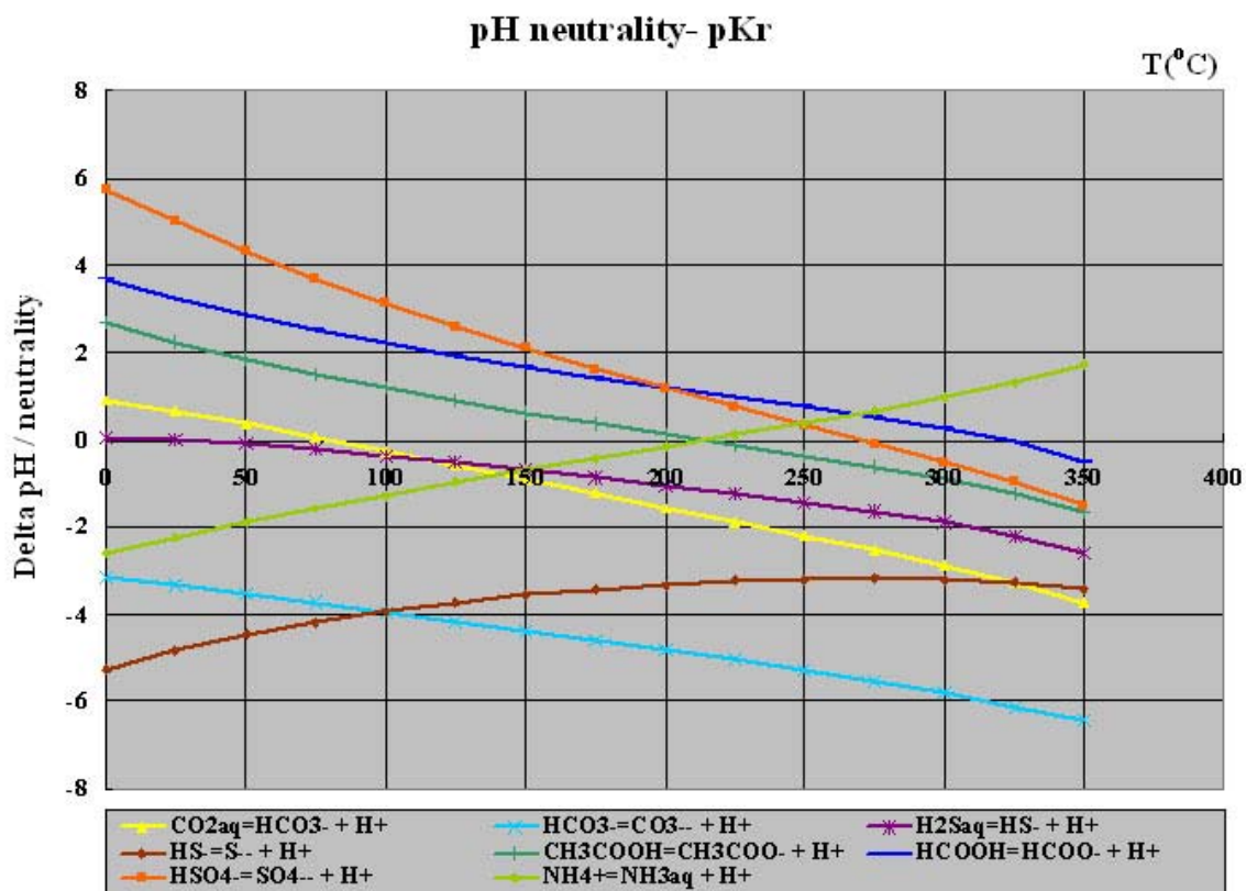
Figure 0-10 Difference of pH of fluids at pH = pKr of different acid-base equilibria versus temperature at water saturation pressure. Delta pH / neutrality = - (1/2) pKw-pKr.
