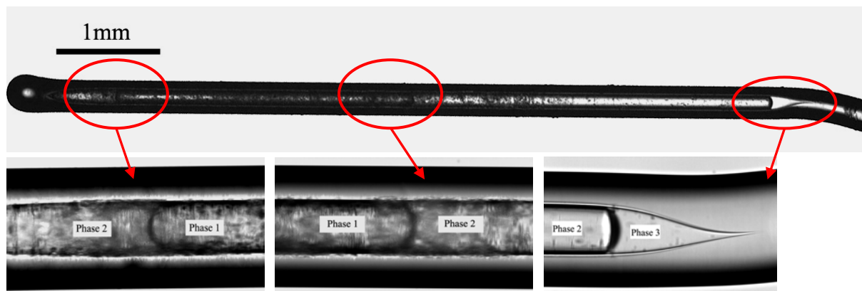
Figure II-22 Microphotographs of the capillary at ambient temperature after heating in the oven. Phase 2 and Phase 3 are two non-colored liquid phases and Phase 1 is vapor phase.
