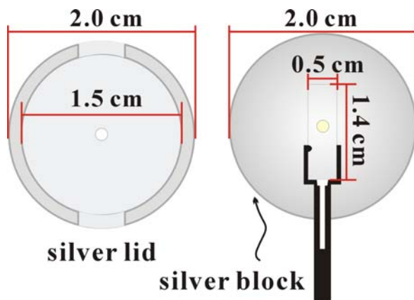
Figure I-3 Sketch of modified silver lid and sample holder and carrier designed for capillary sample.
