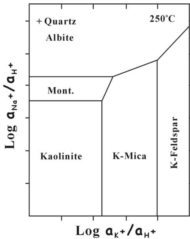
Figure 0-7 Activity diagram for the equilibria of principal mineral phases as a function of pH in the system \text{Na}_2\text{O}-\text{K}_2\text{O}-\text{Al}_2\text{O}_3-\text{H}_2\text{O} at 250 °C at saturation pressure (Henley et al., 1984).
