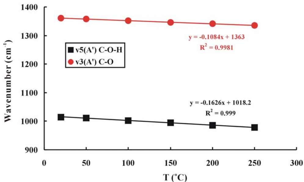
Figure II-11 Variation of v5(A') C-O-H and v3(A') C-O wavenumbers versus temperature. Spectra were collected from fluid inclusion.
