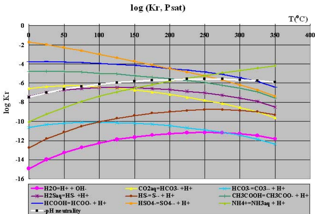
Figure 0-9 Variation of equilibrium constants of acid-base equilibria as a function of temperature along the saturation curve of pure water ( P = P_{sat} at T ). Data are calculated from Program OrganoBioGeoTherm (V. 1.52) written by John J. Donovan.
