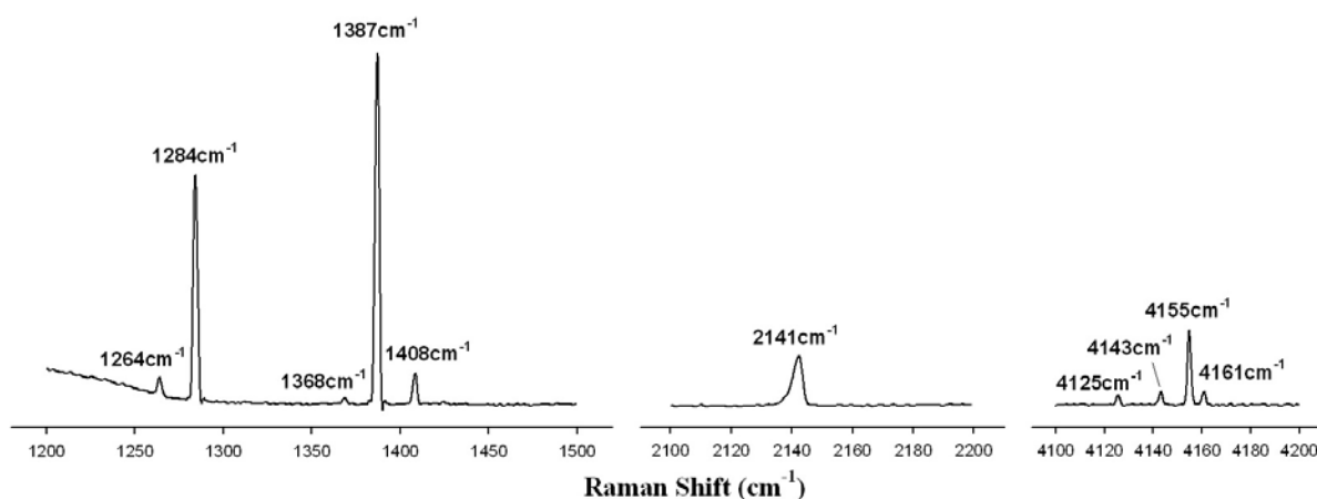
Figure II-30 The Raman spectra of vapour phase in capillary after heating in the microthermometric stage. Bands 1284\text{ cm}^{-1} and 1387\text{ cm}^{-1} : \nu_1\text{-}2\nu_2 Fermi resonance of \text{CO}_2 . Bands 1264\text{ cm}^{-1} and 1408\text{ cm}^{-1} : hot bands of \text{CO}_2 . Bands 1368\text{ cm}^{-1} : the isotopic splitting of
