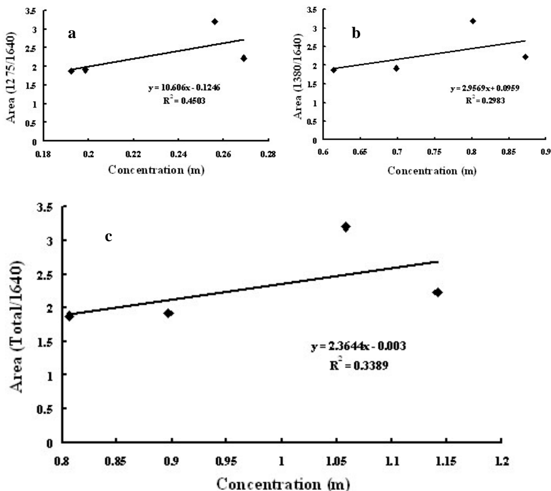
Figure III-5 Relationships between the concentration of \text{CO}_2 dissolved in water and the area ratios of bands of \text{CO}_2 dissolved in water at 1275\text{ cm}^{-1} and 1380\text{ cm}^{-1} obtaining from the analysis of standard capillaries; a. area ratio(1275/1640); b. area ratio(1380/1640); c. area ratio(Total/1640).
