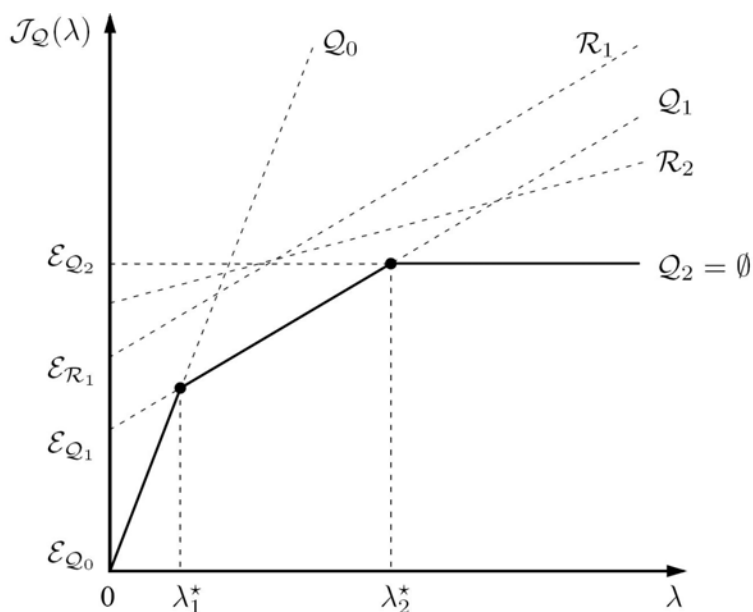
FIGURE 3.1 – Representation of a few lines \lambda \mapsto \mathcal{J}_{\mathcal{Q}}(\lambda) = \mathcal{E}_{\mathcal{Q}} + \lambda \|\mathbf{x}_{\mathcal{Q}}\|_0 for different supports \mathcal{Q} . Note that two lines \mathcal{J}_{\mathcal{Q}} and \mathcal{J}_{\mathcal{Q}'} may coincide. The optimal cost function \lambda \mapsto \mathcal{J}(\lambda) is represented in plain line. It can be interpreted as the “concave envelope” of all lines \lambda \mapsto \mathcal{J}_{\mathcal{Q}}(\lambda) (for all possible supports \mathcal{Q} ). Here, the solution path is described by supports \mathcal{Q}_0 (and the possible other sets yielding the same line) for \lambda < \lambda_1^* , \mathcal{Q}_1 (of lower cardinality) in (\lambda_1^*, \lambda_2^*) , and \mathcal{Q}_2 = \emptyset for \lambda > \lambda_2^* . The supports \mathcal{R}_1 and \mathcal{R}_2 are such that \forall \lambda, \mathcal{J}_{\mathcal{R}}(\lambda) > \mathcal{J}(\lambda) .
