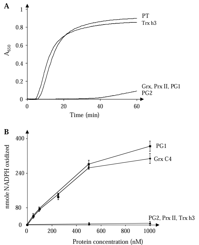
Fig. 7. Specific Trx or Grx activity tests. (A) Insulin reduction was followed at 650 nm in the presence of 500 \mu M DTT and the various proteins at 5 \mu M. (B) DHA reduction activity in function of protein concentration was measured by following NADPH oxidation at 340 nm in a coupled reaction system.
