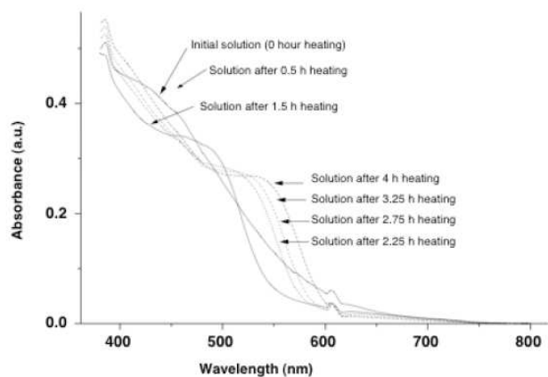
Fig. (2). Growth of TGA-stabilized CdTe QDs monitored by UV-vis absorption spectroscopy during 5 h at 100°C.
