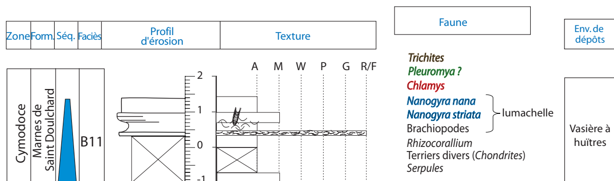
Figure 4.21 Coupe de Saint-Doulchard
