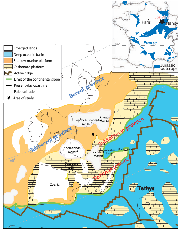
Fig. 1 Paleogeographic map of the Early Kimmeridgian of Western Europe (simplified from Cecca et al. 1993), paleobiogeographical provinces and location of the studied section
