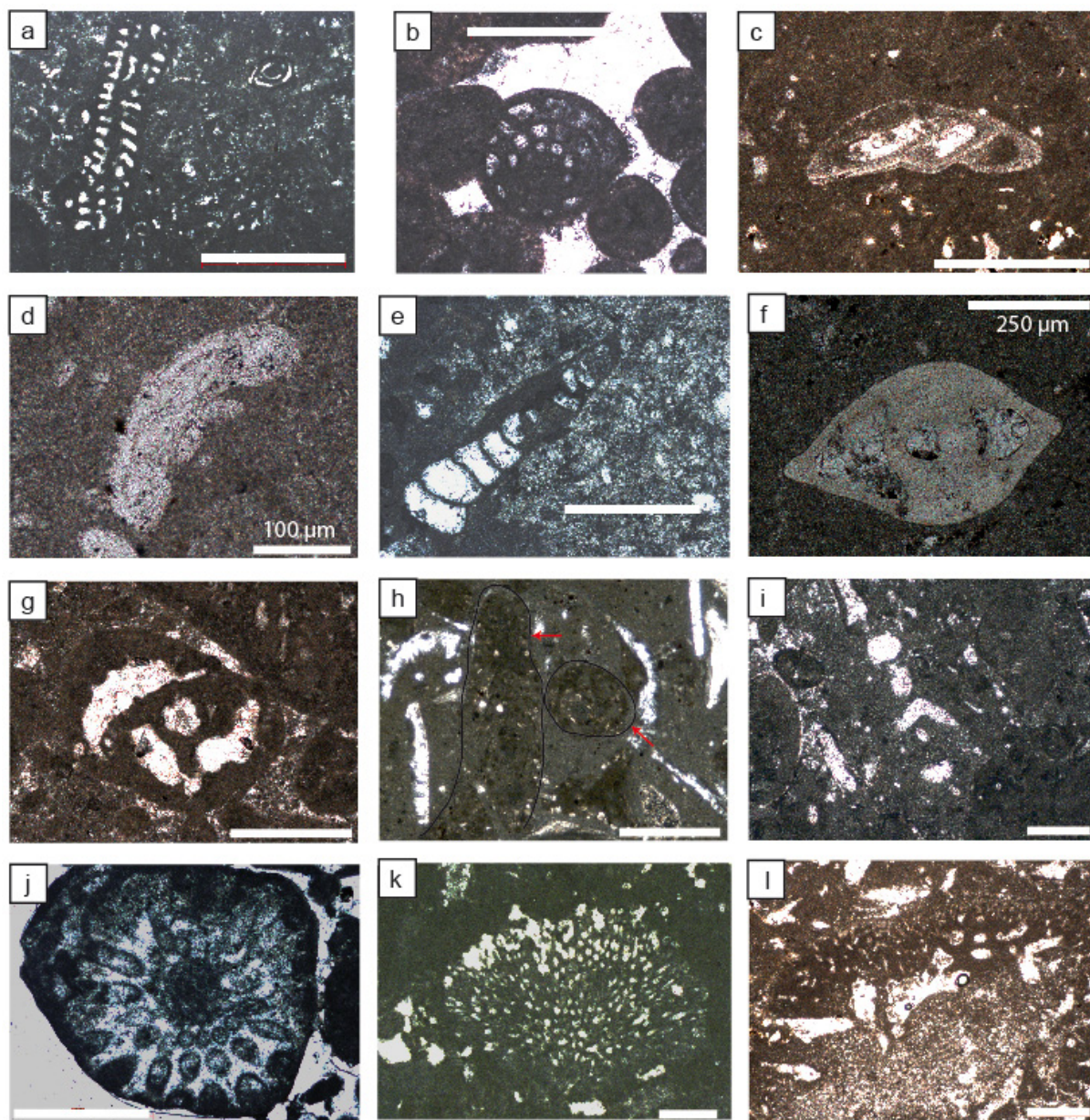
Fig. 6 Microfossils of the Upper Oxfordian-Lower Kimmeridgian from the Gudmont-Villiers section. a Labyrinthina mirabilis Weinschenk and Labalina (Calcaires crayeux de Gudmont Formation). b Nautiloculina oolithica Mohler (CCG Formation). c Mohlerina basiliensis (Mohler)(Calcaires À serpules de Gudmont Formation). d Hungarillina pedunculata Blau & Wernli (Calcaires À serpules de Gudmont Formation). e Troglotella incrustans Wernli & Fuchs in Cladocoropsis mirabilis Felix (Calcaires crayeux de Gudmont Formation). f Pink Lenticulina (Calcaires à astartes Formation). g , i Everticyclammina virguliana (Koechlin) (CCG Formation & Oolithe de Lamothe Formation). h Alveosepta jaccardi (Schrodt) (CCG Formation). j Dasycladacean ( Salpingoporella annulata Carozzi?) G6. k Cayeuxia pia Frolo (G 9 ). l Lithocodium aggregatum Elliott (Calcaires crayeux de Gudmont Formation). When the scale is not precised, the segment measures 500 µm.
