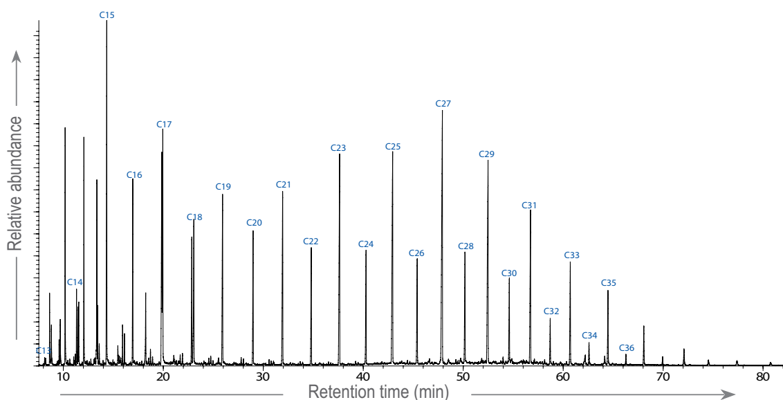
Fig. 5.9 Bimodal distribution of the n -alkanes : example of the sample F539 ( m/z 57).
