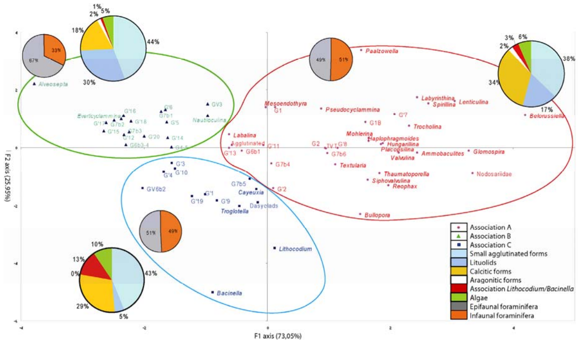
Fig. 7 The faunal associations, A, B and C determined by MCA, HAC and DA. Pie-diagrams: microhabitats (epi- or infaunal foraminifera) and shell composition of foraminifera, algae and Lithocodium/Bacinella association
