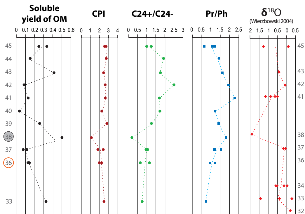
ig. 5.7. Soluble yield of the organic matter, Carbon Preference Index (CPI), n -C24 +/ n -C24- ratio, Pristane/Phytane ratio and δ 18 O (values of Wierzbowski 2004) of the samples of clay and limestone beds of the Flodigarry section. The bed rimmed by grey circle is the bituminous bed, the bed 36 rimmed in orange is the boundary bed between Oxfordian and Kimmeridgian stage proposed by Wierzbowski et al. (2006).
