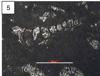
5. Troglotella incrustans (G'2)
