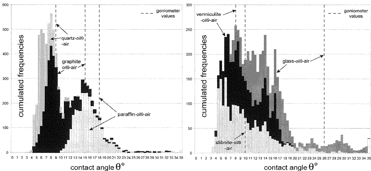
Fig. 9: Frequency histograms of the contact angles calculated with the CSLM 3D models for the different three phase systems. Bars with different patterns correspond to the different systems and the dashed lines indicate the respective values of the contact angles determined with the goniometric method.
