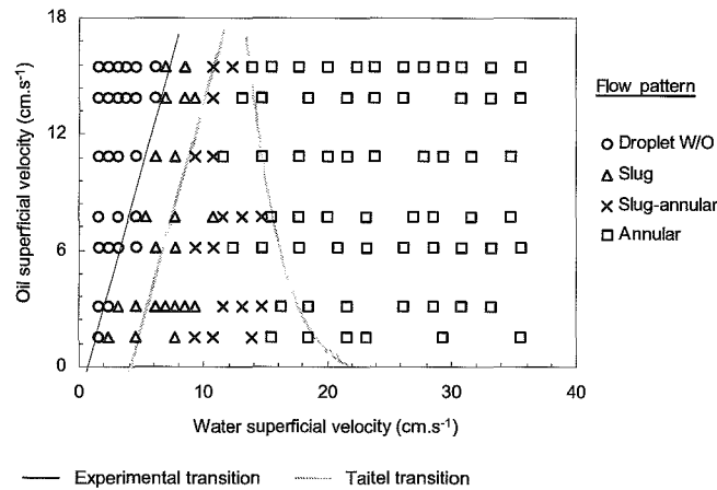
Figure 4a: Flow pattern transitions: microchannel initially saturated with oil.
