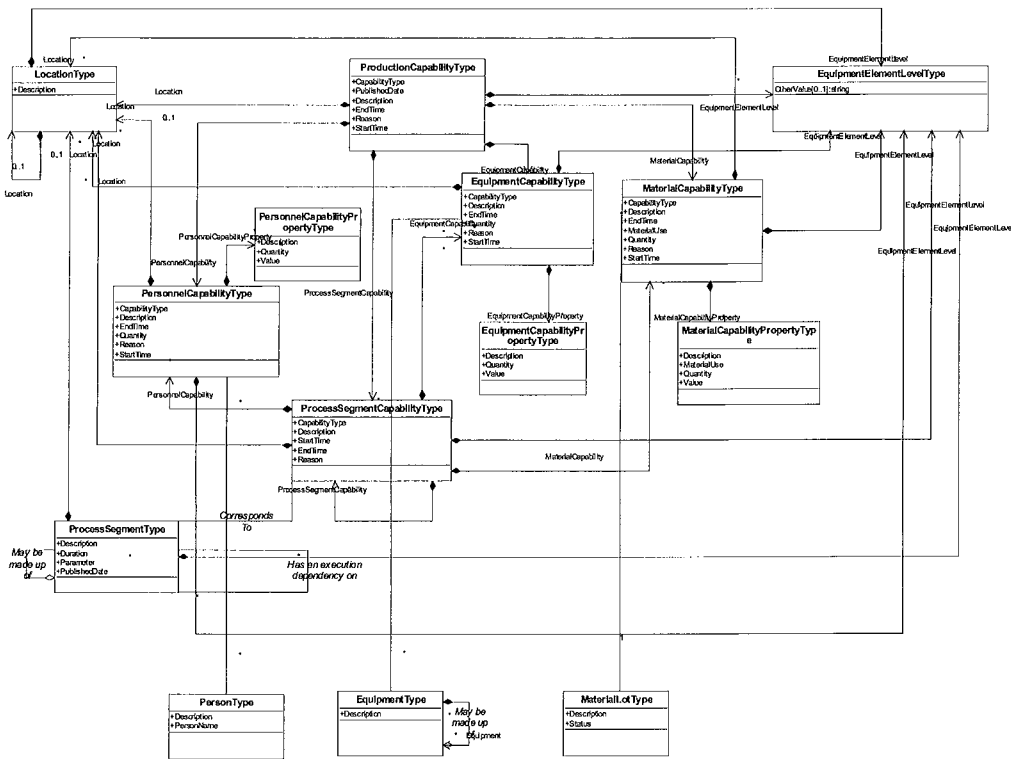
Figure 6.7 - B2MML schemas definitions for production capability
