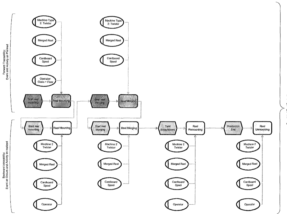
Figure 9.11 - Completed reel production EPC model
