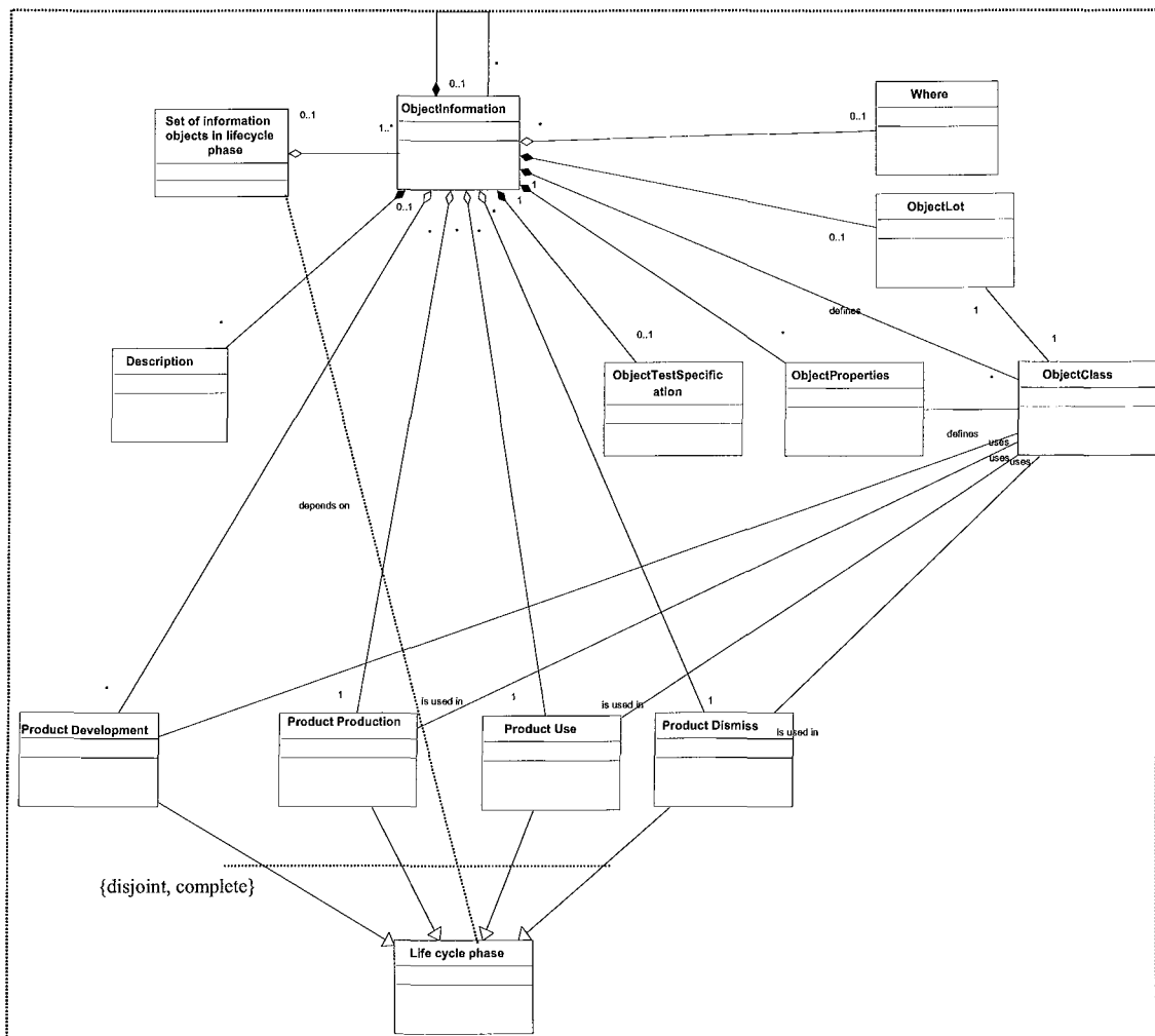
Figure 8.11 - ObjectInformation model
