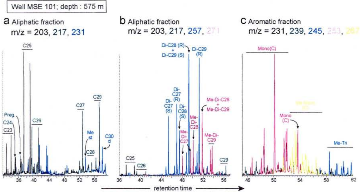
Figure IV.8. (a) Distribution of steranes and methylsteranes ( m/z 203, 217, 231). (b) Distribution of steranes, diasterenes and methyl-diasterenes ( m/z 203, 217, 257, 271). (c) Distribution of aromatic steroids ( m/z 231, 239, 245, 253, 267). Preg. : pregnane; C23 to C29 : regular steranes having from 23 to 29 carbon atoms; C30d : dinosterane; Mest : methylsterane; Di-C27 to Di-C29 : diasterenes having from 27 to 29 carbon atoms; Me-Di-C27 to Di-C29 : methyl-diasterenes having from 27 to 29 carbon atoms; Mono(C) : monoaromatic steroids; Me-Mono(C) : monoaromatic methylsteroids; Me-Tri : triaromatic methylsteroids.
