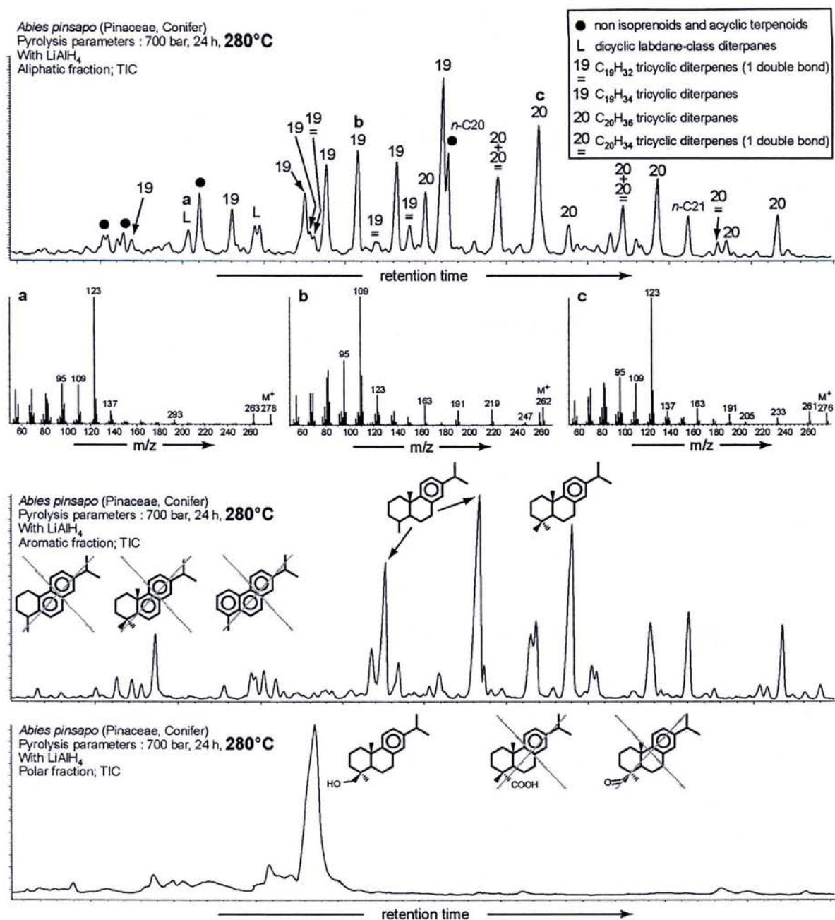
Figure VII.6. Partial chromatograms (diterpane retention time window) of aliphatic, aromatic and polar fractions of pyrolysis product of Abies pinsapo at 280°C with addition of metal hydride (LiAlH 4 ). Mass spectra of aliphatic compounds noted a (labdane), b (norabietane) and c (abietane), are shown for the aliphatic fraction.
