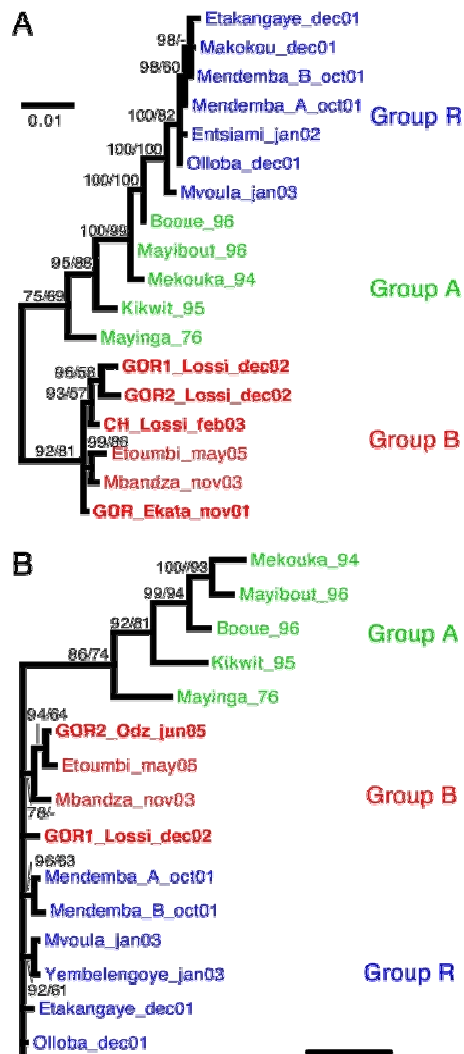
Fig. 1. Phylogenetic relationships inferred from GP gene (A) and NP gene (B) sequences that show relationships among all of the ZEBOV isolates. Viruses derived from wild ape carcasses are shown in bold. Values above branches represent Bayesian posterior probabilities and ML bootstrap scores (both at percentages). Colors identify three genetic groups of ZEBOV: green, group A; red, group B; blue, recombinant group R.
