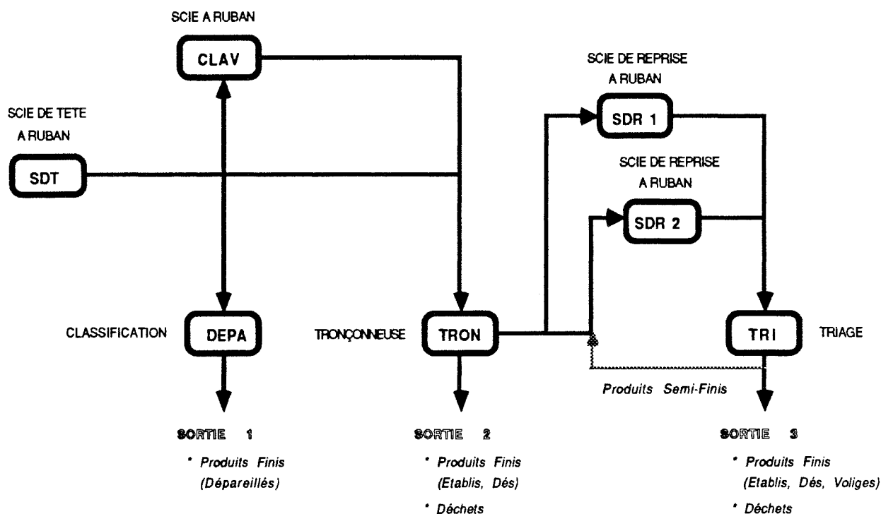
Figure 5.1: Système de Production Simulé (Scierie "A")
