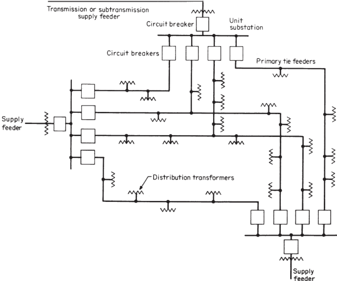
Figure 2.2: Primary network. Sectionalizing devices on feeders not shown.
