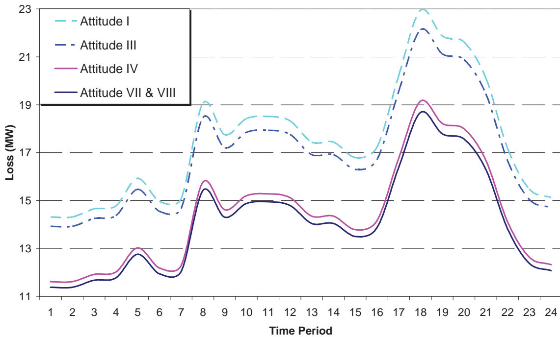
Figure 4.30: Total system losses versus time period in attitudes I, III, IV, VII&VII.
