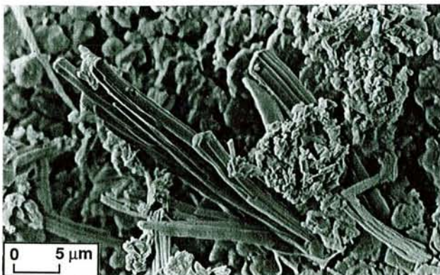
Halotrichite
