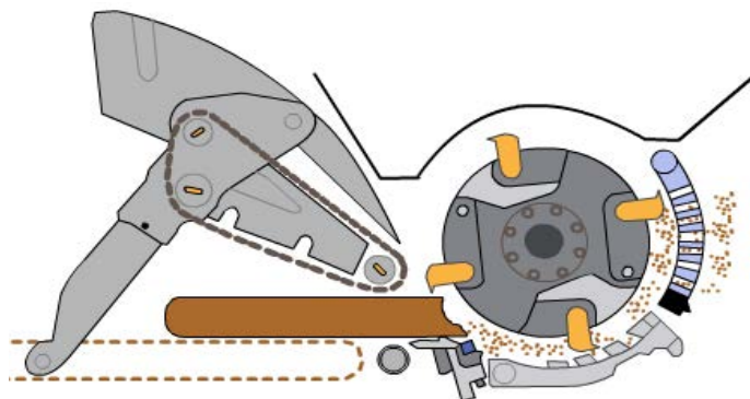
Figure 40: Tambour à marteaux (FORUS)
