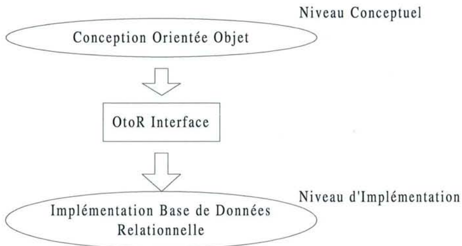
Figure 2. L'interface Object-to-Relationnel
