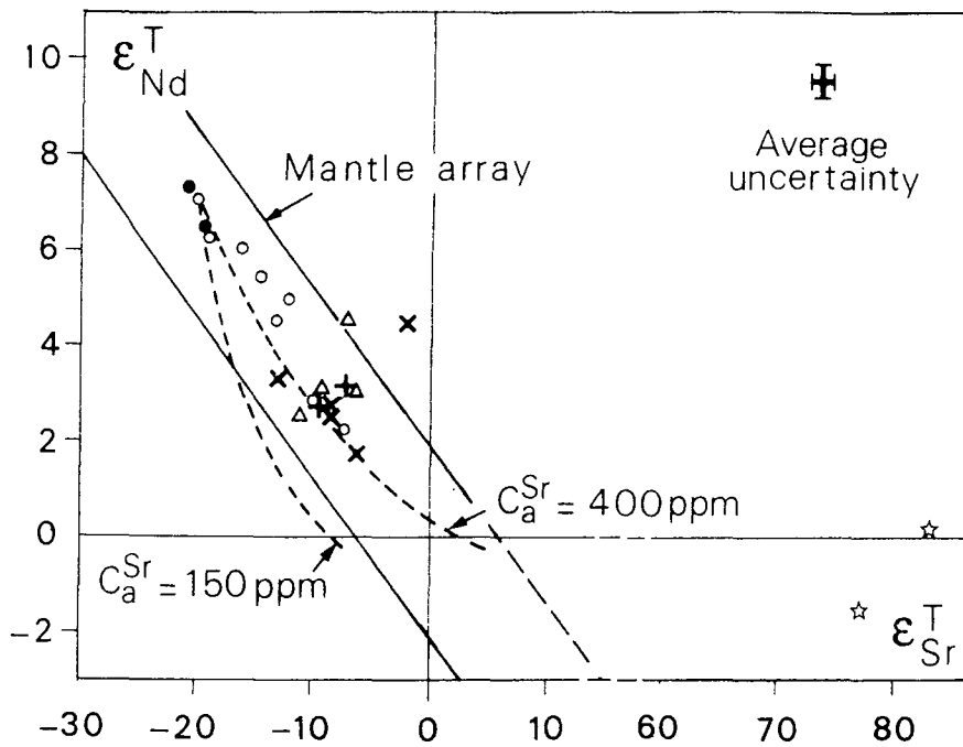
Figure V.9 - \epsilon_{Nd}^T vs \epsilon_{Sr}^T plot for the five main rocks types of the Tichka complex.
