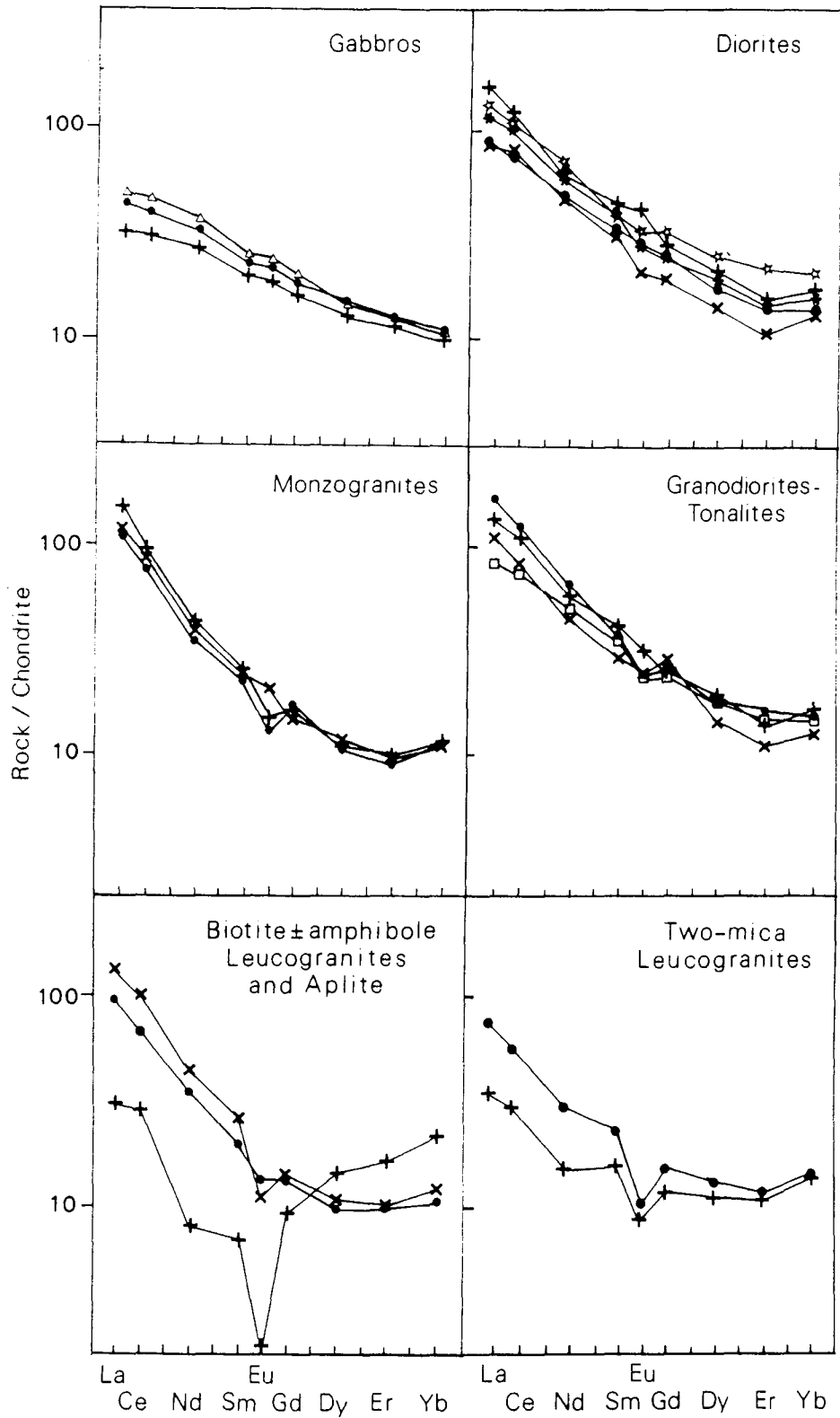
Figure V.6 - Chondrite - normalized REE patterns of the rock - types from the Tichka complex Normalizing values from Evensen et al. [65].
