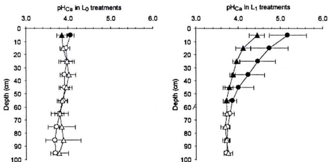
Figure 2: Soil \text{pH}_{\text{Ca}} profiles for each treatment at the end of the experiment. Mean and confidence interval ( P < 0.05 ) on five plots are presented for each sub-treatment M ( -\circ- ) and F ( -\Delta- ) both in L_0 (no-lime) and L_1 (lime) treatments. Filled points correspond to statistically significant differences between the two means ( P < 0.05 ).
