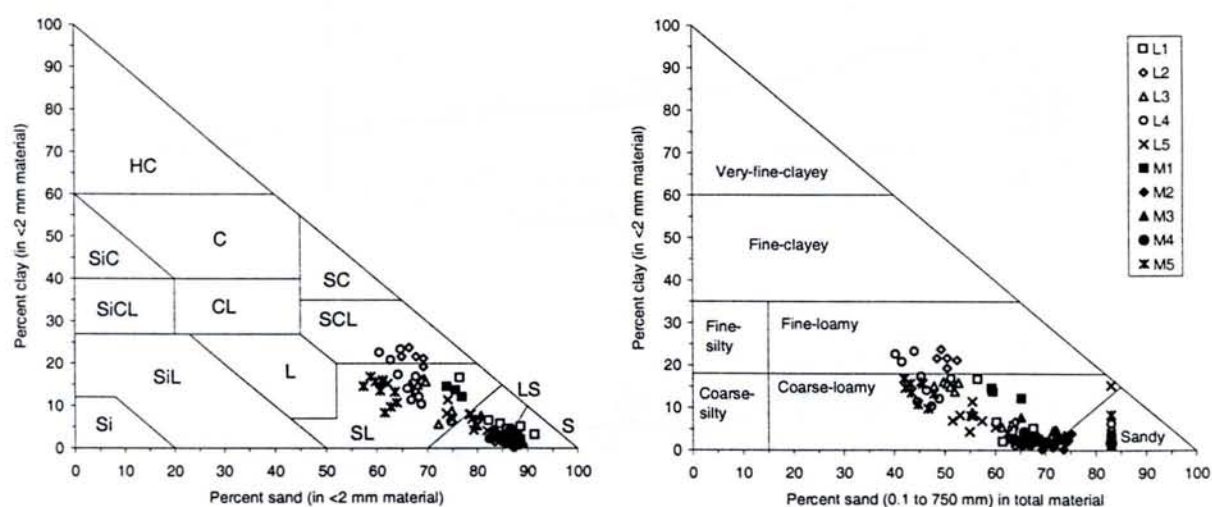
Figure 3: Repartition of studied soil in soil texture classes triangle (left) and family particle-size classes triangle (right). Abbreviations for the texture classes are HC, heavy clay; C, clay; SiC, silty clay; SiCL, silty clay loam; CL, clay loam; SC, sandy clay; SiL, Silt Loam; L, loam; SCL, sandy clay loam; SL, sandy loam; Si, silt; LS, loamy sand; S, sand.
