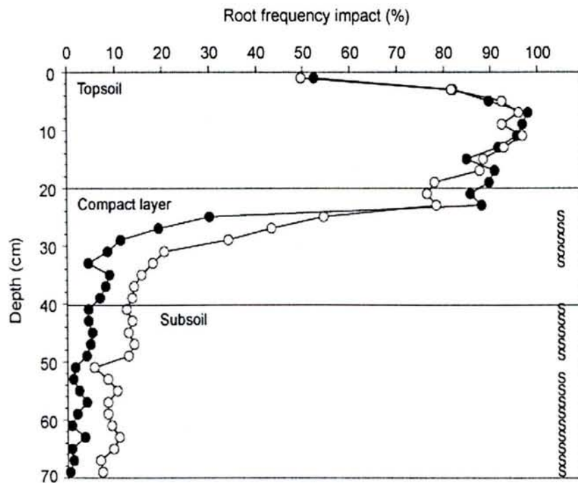
Figure 3: Root frequency impacts of a maize crop (in the third year of the study). Stylo/maize rotation (—●—) and continuous stylo treatment (---○---). "S" indicates significant difference for the considered depth (n=5, P<0.05 ).
