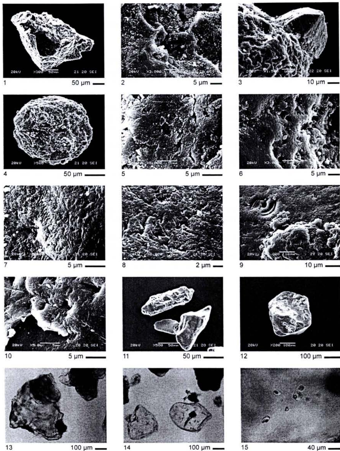
Plate 1 : Exoscopic and endoscopic features of the quartz sand grains.
