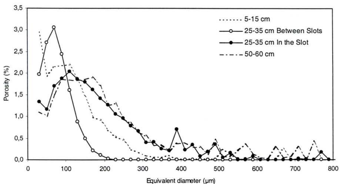
Figure 2: Pore size distribution from image analysis.
