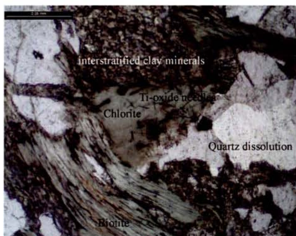
Fig. 2.35. Chlorite (pycnochlorite) and interstratified minerals neof ormation, accompanied by quartz dissolution and biotite alteration (DDH-625-140 m, Karku deposit, ore zone III) Microphotograph scale - 0.25 mm
