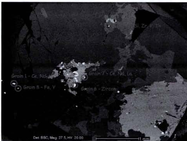
Fig. 2.89. Abundant REE-bearing accessory minerals included in biotite in the even-grained biotite granite (sample 5-04-01, Pitkyaranta area). BSEM image, photomicrograph scale – 1 mm
