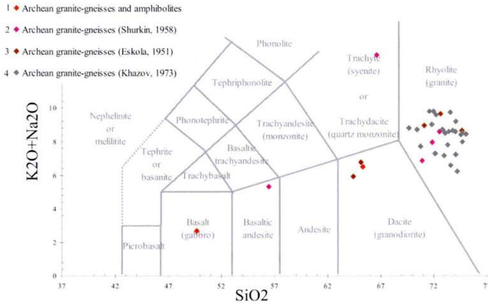
Fig. 2.12. Early Archean rocks from the dome structures of the Northern Ladoga area in the SiO 2 vs. K 2 O + Na 2 O classification diagram. 1 - 4: chemical analysis data of the Archean granite-gneisses and amphibolites after 1) present work, 2) Shurkin, 1958; 3) Eskola, 1951; 4) Khazov, 1973.
