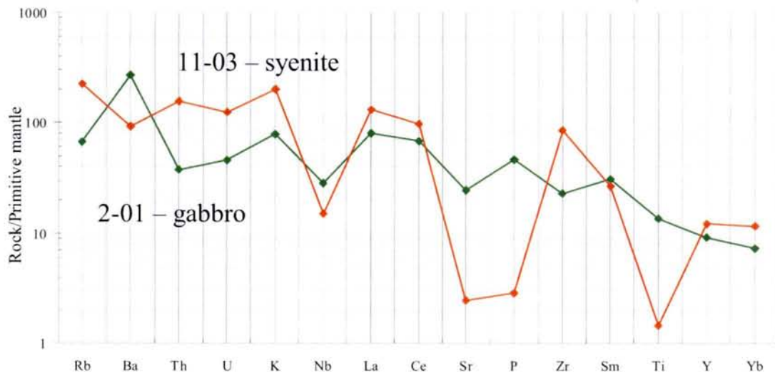
Fig. 4.21. Primitive mantle normalized trace element patterns of the Valaam sill rocks (spidergram type after Holm (1979); primitive mantle composition after Wood et al (1980)
