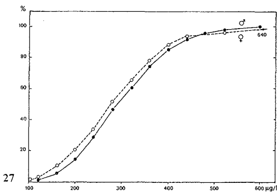
Curve 25. Erythrocyte glutathion reductase activation.
