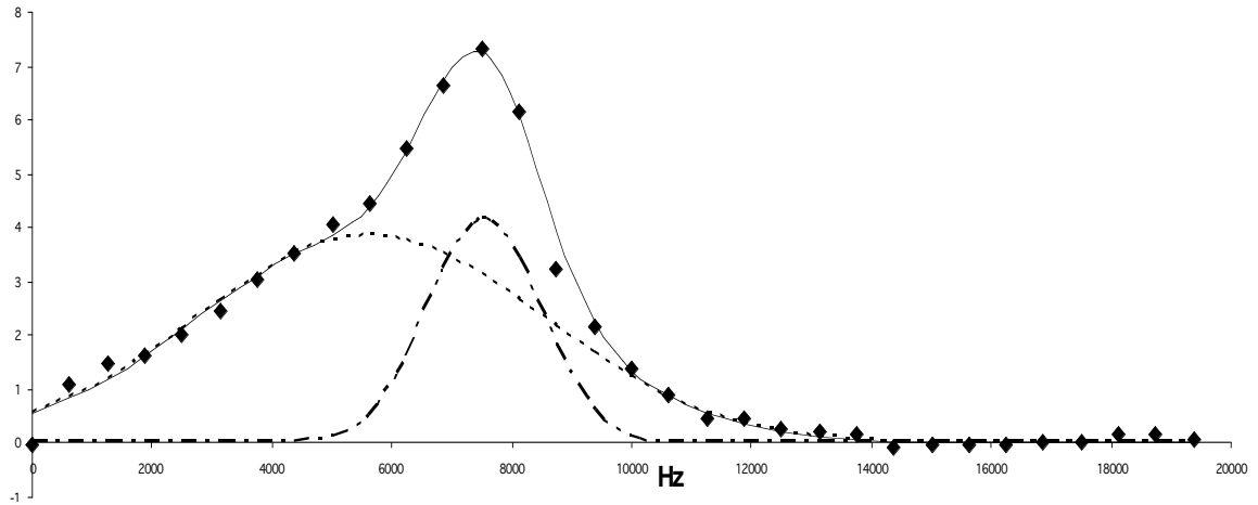
Figure 4: The spectrum resulting from the Fourier transform of a nutation curve (after subtraction of the steady state value) obtained at moderate rf amplitude ( \gamma B_1/2\pi = 7500 Hz). Diamonds represent experimental data. In addition to the expected signal close to \nu_1 = \gamma B_1/2\pi (the dashed peak), it can be seen that the Lorentzian of figure 3 has been substituted by a signal (dotted line) at a frequency smaller than \nu_1 . The solid line is a plot of the superposition of the dotted and dashed signals. The peak decomposition has been achieved in the time domain as explained in the text.
