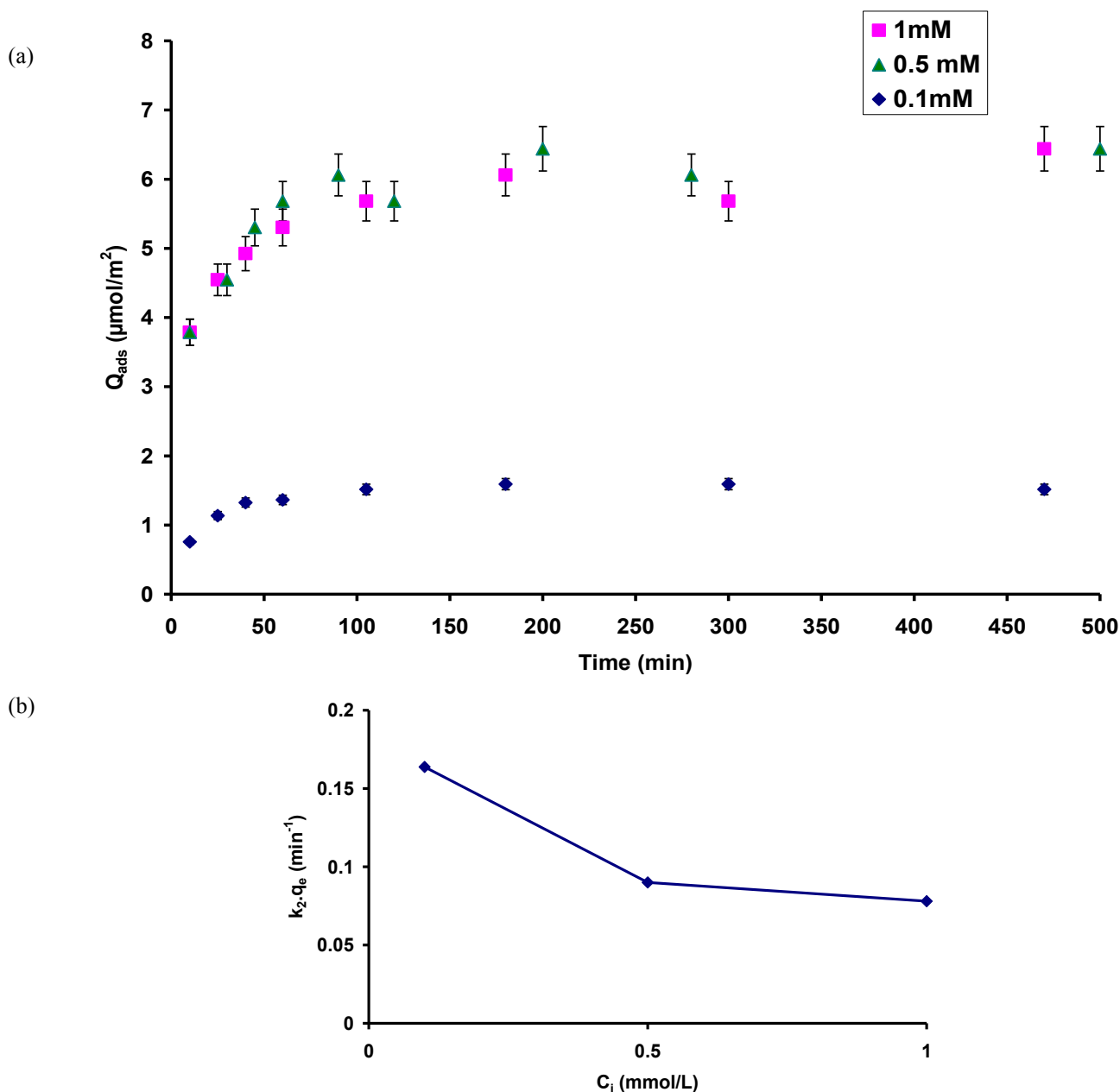
Figure D-22 : (a) Adsorption of gentisic acid onto HCS versus time at 0.1, 0.5 and 1mM of initial GA concentration, at pH 3 and a background electrolyte of 10 mM NaCl. Particle concentration was 1g/L of HCS, temperature was constant at 20°C. Error bars represent standard deviations based on triplicate analyses. (b) Sorption rate constant reported to the maximum sorbed amount ( k_2 \cdot q_e ( \text{min}^{-1} )) versus initial solute concentration (mM).
