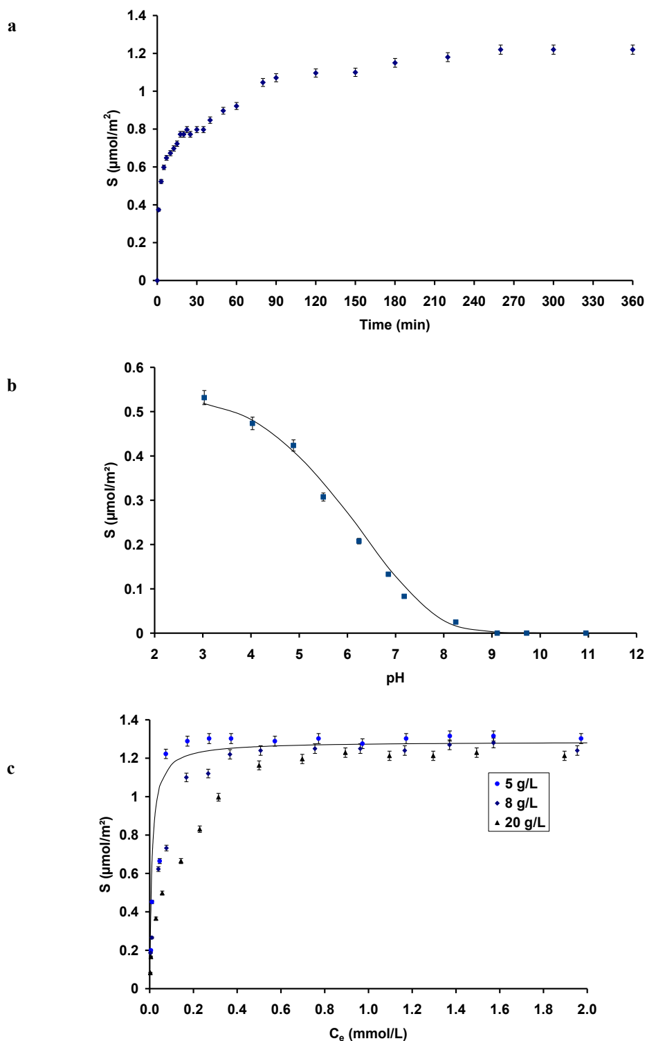
Figure D-10 : a) Batch adsorption of SA onto GCS versus time at pH 4.0±0.1. [SA] = 1 mmol/L; [GCS] = 8 g/L; T = 20±1 °C; 10 mmol/L NaCl as supporting electrolyte. b) Sorption data of salicylate versus pH. [SA] = 0.06 mmol/L; [GCS] = 8 g/L; T = 20±1 °C; 10 mmol/L NaCl as supporting electrolyte. Solid line represents surface complexation model. c) Sorption isotherms of salicylate to GCS at different solid loading: 5, 8 and 20 g/L; pH 4±0.1, T = 20±1 °C and 10 mmol/L NaCl as supporting electrolyte. Solid line represents SCM model of the data at 8 g/L. For all data, error bars represent standard deviations based on triplicate analyses.
