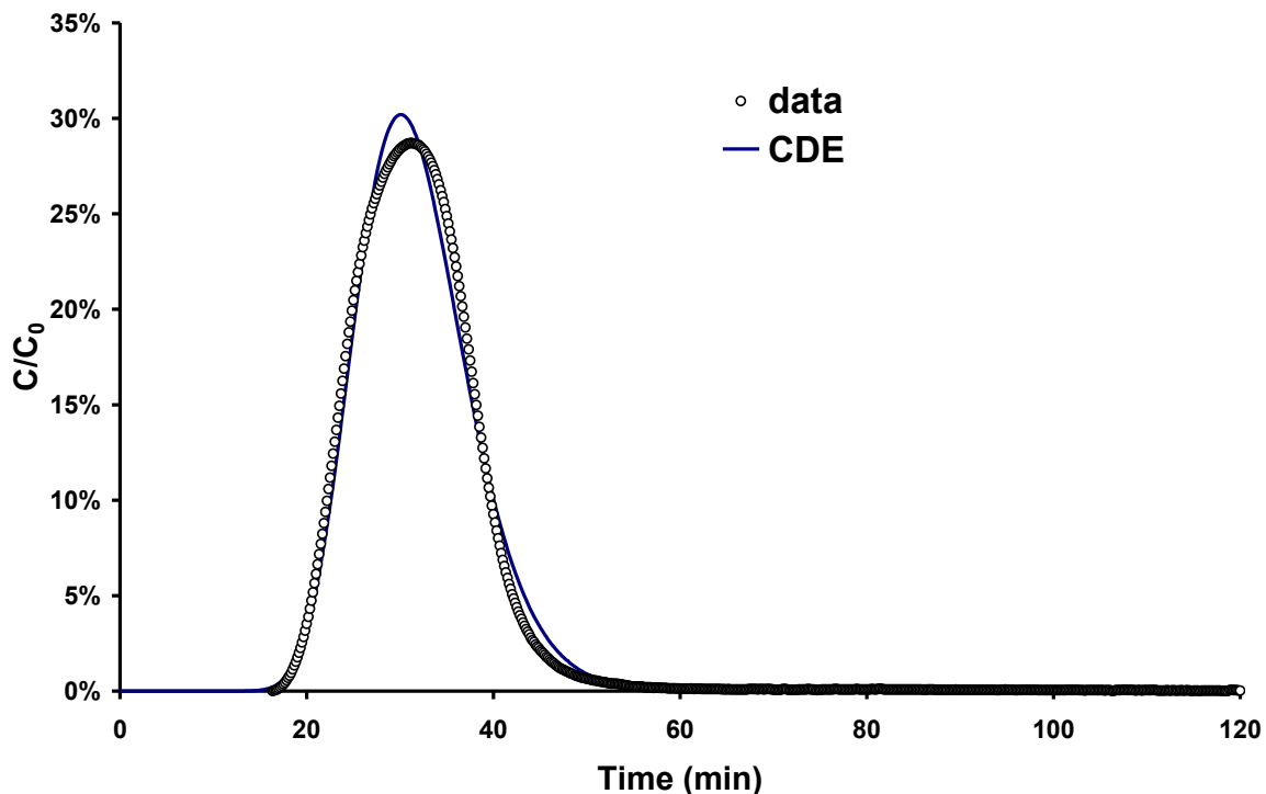
Figure D-25 : Breakthrough curve of the Br - non-reactive tracer for the HCS packed column, experimental data and calculations based on the CDE model (Convective-Dispersion equation).
