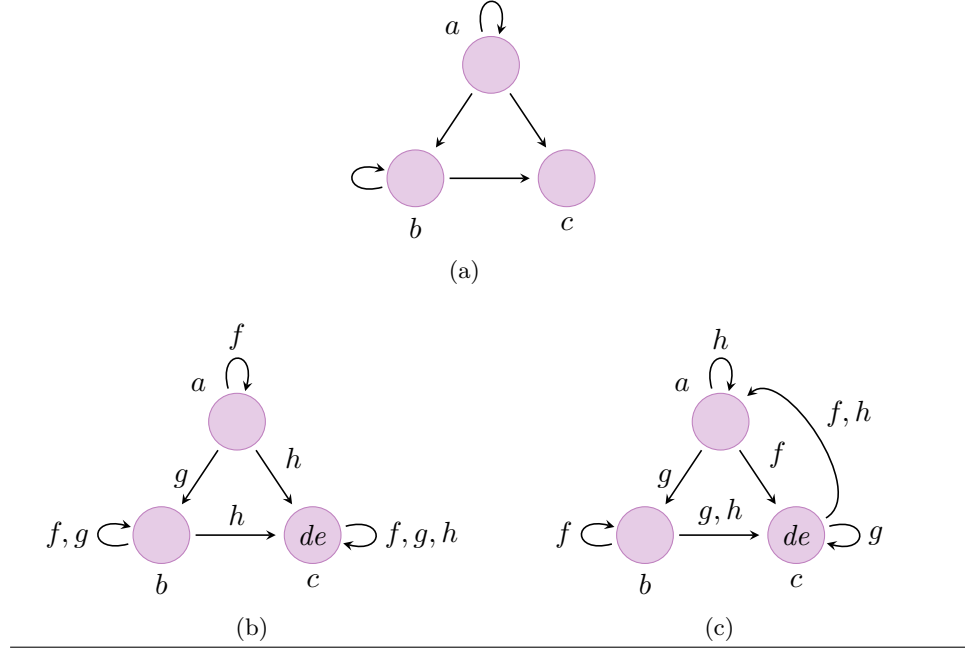
Figure 6.1: A relational structure (a) is represented in (b) and (c) using total functions f, g, h and a predicate de .
