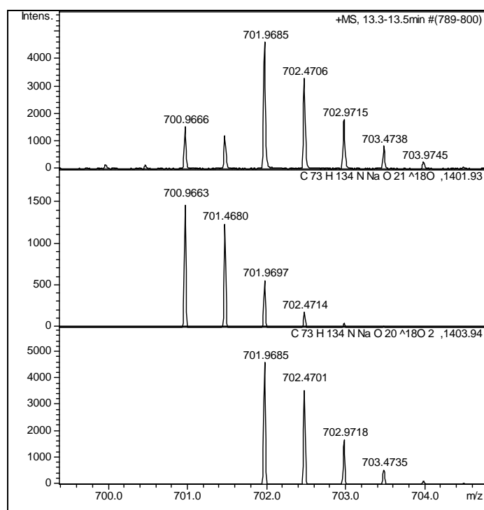
Fig. 14 ESI-TOF mass spectrum of sambomycin A/B labelled with one or two ^{18}\text{O} (on top), corresponding to the sodiated form, and their simulated mass spectra (on bottom).
