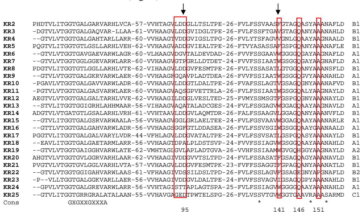
Fig. 34 Amino acid alignments of the KR domains. The consensus sequence at the N-termini was proposed to bind to the NAD(P)H (Aparicio et al. , 1996). The amino acids of the catalytic triad are marked with an asterisk. The boxed amino acids are involved in the stereochemistry of the polyketide. The arrows indicated the residue 95 and 141 specific for the B and A-type alcohol stereochemistry, respectively. At the bottom the amino acid position referred to the KR domain in the DEBS genes are indicated. On the right of the alignment, for each KR domain, the configuration of \alpha -substituents and \beta -hydroxyl groups derived from each precursor are given, according to the nomenclature proposed by Keatinge-Clay (2007). A1= 2R, 3S; A2=2S, 3S; B1=2R, 3R; B2= 2S, 3R; C1=2R.
