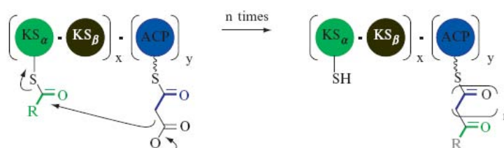
Fig. 24 Type II PKS mechanism: discrete catalytic enzymes are responsible for the chain elongation (from Weissman, 2009). \text{KS}_\alpha and \text{KS}_\beta domains form a heterodimer, in analogy to the modular KS homodimer. The ACP domain is used as anchor for the growing chain (Hertweck et al. , 2007).
