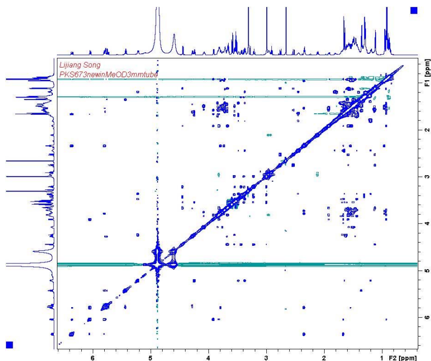
Fig. 13 NOESY spectrum (700 MHz) of sambomycin C/D in d_4 -MeOH.
