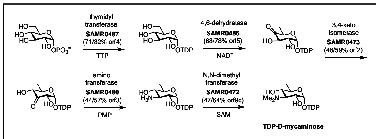
Fig. 41 Schematic representation of TDP-D-mycaminose biosynthetic pathway from an \alpha -D-glucose-1-phosphate. For each enzymatic step, the gene product is indicated in bold. In brackets, the percentages of identity/similarity with the spiramycin enzymes are indicated (Karray et al. , 2007). Abbreviations: TTP, thymidine triphosphate; TDP, thymidine diphosphate; \text{NAD}^+ , nicotinamide adenine dinucleotide; PMP, pyridoxamine 5'-phosphate; SAM, S-adenosyl-L-methionine.
