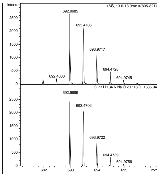
Fig. 16 ESI-TOF mass spectrum of a modified form of sambomycin A/B labelled with one ^{18}\text{O} (on top), generating from the mutant strain ATCC/ \Delta 478, and the simulated mass spectra (on bottom), lacking on oxygen atom.
