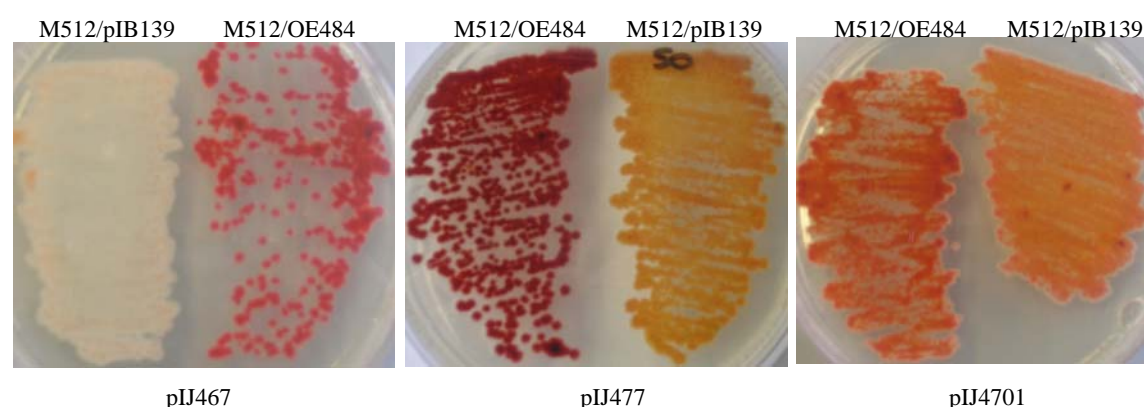
Fig. 67 Undecylprodigiosin-producing colonies by the transformants M512/OE484 containing the recombinant vectors pIJ-R0467, pIJ-R0477 and pIJ-R04701, compared to the transformants M512/pIB139 containing the same plasmids. The transformants are plated on R2YE+25µg/ml thiostrepton. The colour of the colonies can sometimes appear darker because the plates were incubated at 30°C for a longer time.
