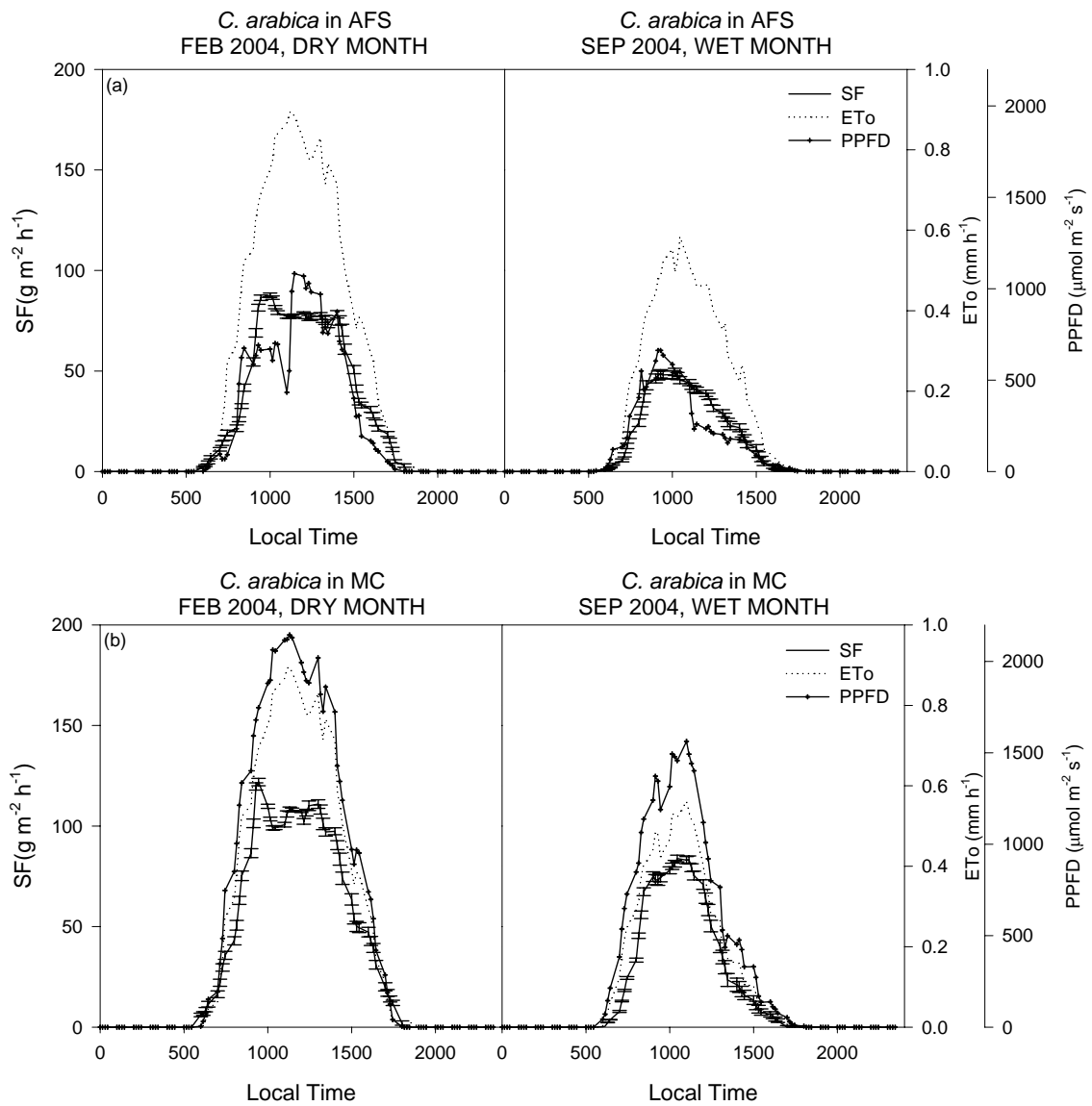
Figure 4. Mean hourly coffee sap flow rate (SF), reference evapotranspiration ( ET_o ; measured in open field) and photosynthetic photon flux density (PPFD) based on ten consecutive days and four coffee plants in AFS (a) or in MC (b) for a dry month (February) and wet month (September) in San Pedro de Barva, Costa Rica (values \pm sd are means over periods of 15 min).
