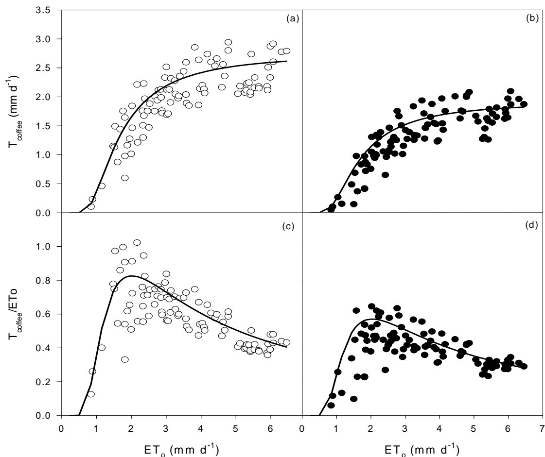
Figure 19. Relationships between daily coffee transpiration (a&b) and coffee transpiration over ET_0 (c&d) versus daily ET_0 (FAO, 1998) in MC (left panels) and in AFS (right panels) at San Pedro de Barva, Costa Rica. (Daily transpiration values are extrapolations to ha from four coffee plants).
