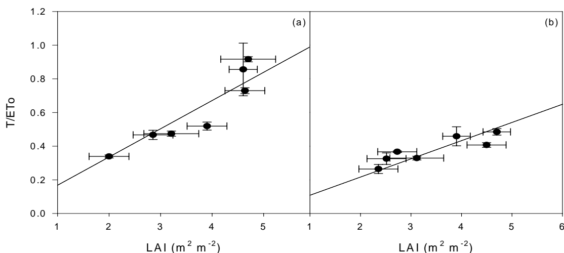
Figure 22. Relationships between R (ratio of coffee transpiration over E_{To} ) and LAI in MC (a) and in AFS (b) at San Pedro de Barva, Costa Rica. (Values represent daily averages for one to two weeks of measurements. MC: r^2=0.98 , R=0.17*LAI ; AFS: r^2=0.98 , R=0.11*LAI ).
