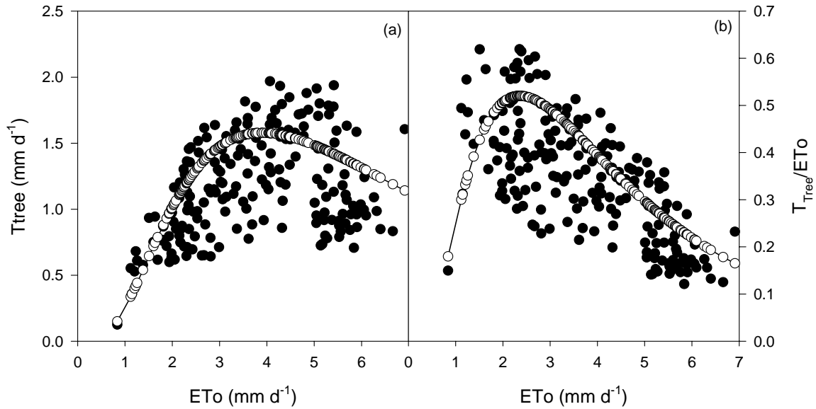
Figure 3. Relationships between reference evapo-transpiration ( ET_o ) and (a) daily transpiration ( T ) and (b) the ratio T/ET_o of I. densiflora in an agroforestry system at San Pedro de Barva, Costa Rica.
