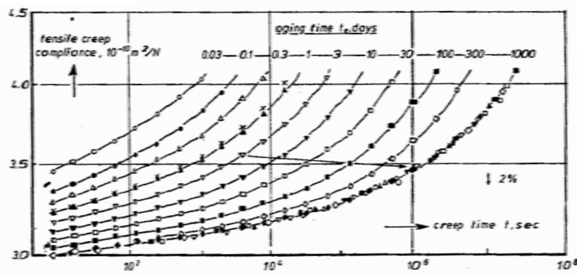
Figure 1.1: Small-strain tensile creep curves of PVC quenched from 90^\circ\text{C} to 20^\circ\text{C} . The arrow indicates the almost horizontal shift performed to obtain the data collapse. The crosses were found when, after 1000 days of ageing, the sample was reheated to the original temperature, requenched and then remeasured for t_e = 1 day. The image is taken from [224].
