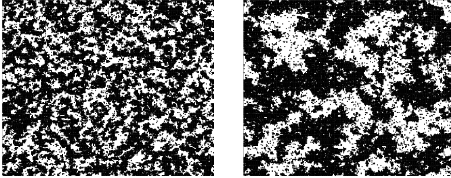
Figure 1.7: Snap-shot of a Monte-Carlo simulation of the Ising model quenched onto the critical point. White areas have spin up, black areas spin down. The left picture shows the system a relative short time after the quench, the right picture at a later stage. Both pictures courtesy of M. Pleimling
