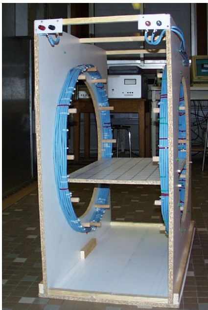
(a) Helmholtz
