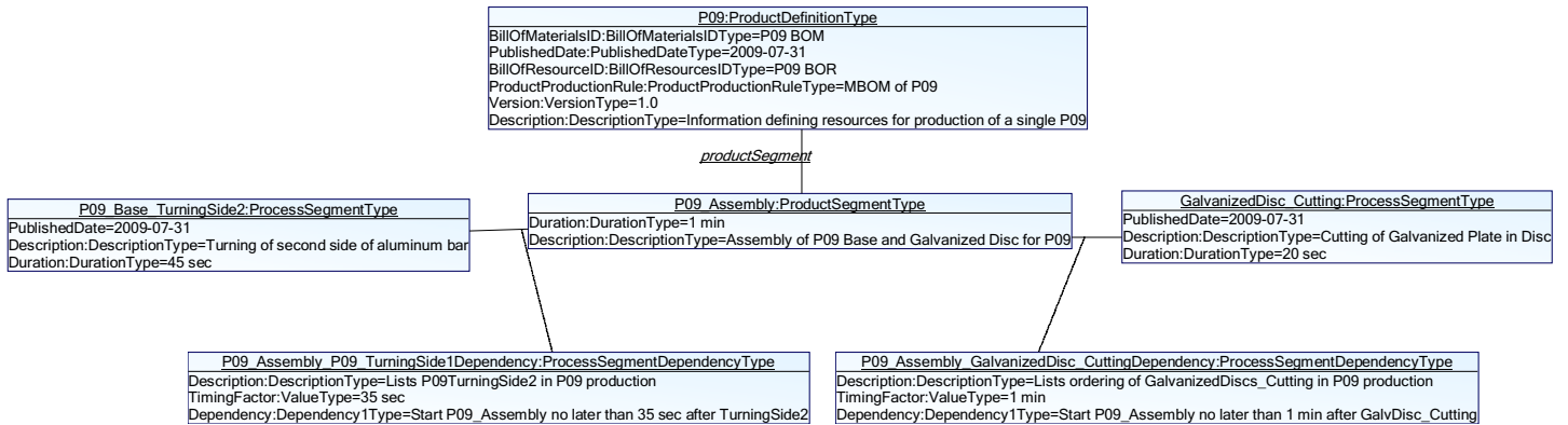
Figure 42 (c) – The MBOM in the Product Ontology
