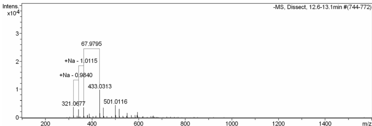
Figure 2.12. APCI-MS spectrum of the raw SFA_1 fraction eluted at 12.8 minutes and analyzed in negative mode.
