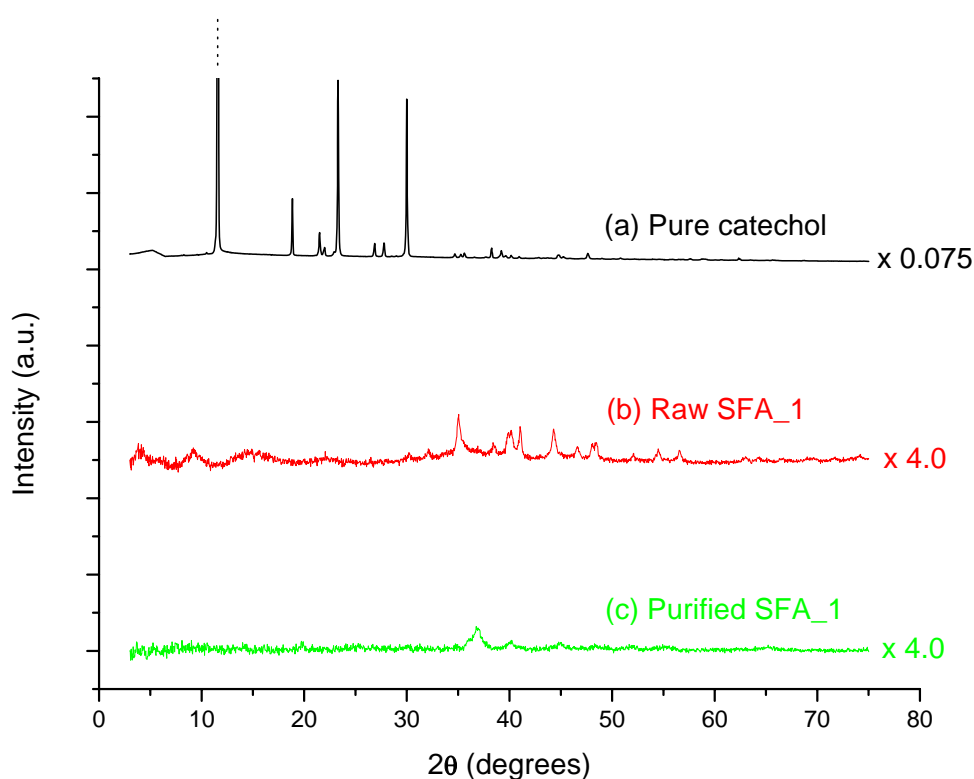
Figure 2.2. X-ray diffraction spectra of crystalline catechol (a), of a raw mixture of SFA_1 and Na-catecholate salts (b), and of amorphous SFA_1 after extraction (c) – see text.
