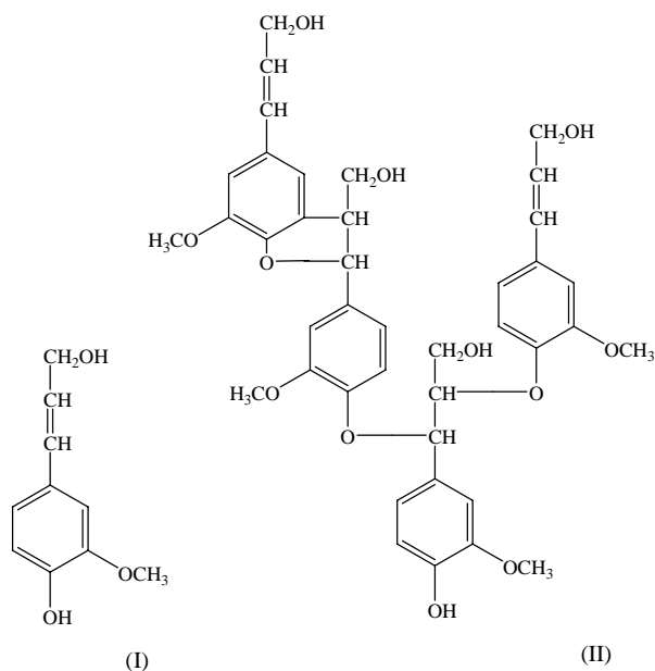
Figure 2.17. Molecular structures of coniferyl alcohol (I), the constitutive monomer of lignin, and of tetralinol (II), an oligomer formed by polymerization of (I) – Fengel and Wegener, 1983.
