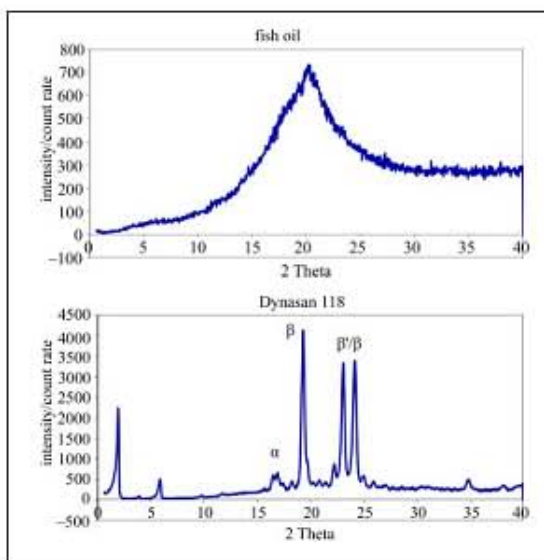
Fig. 4: X-ray diffraction pattern of the bulk materials fish oil and Dynasan 118 (explanations in the text)
