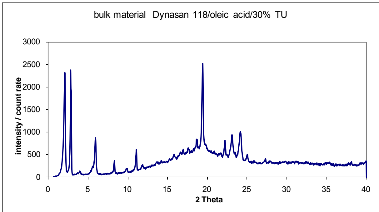
Bulk material: Dynasan 118/oleic acid/TU (35/35/30) (m/m)
