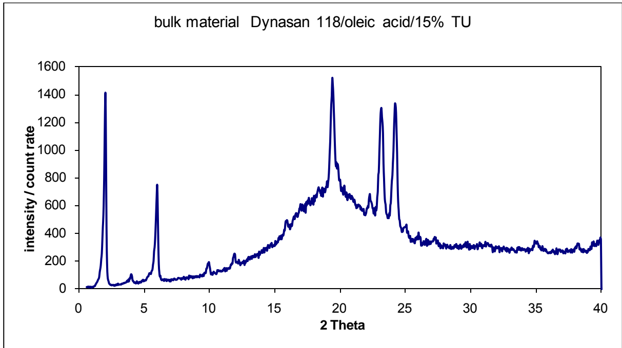
Bulk material: Dynasan 118/oleic acid/TU (42,5/42,5/15) (m/m)
