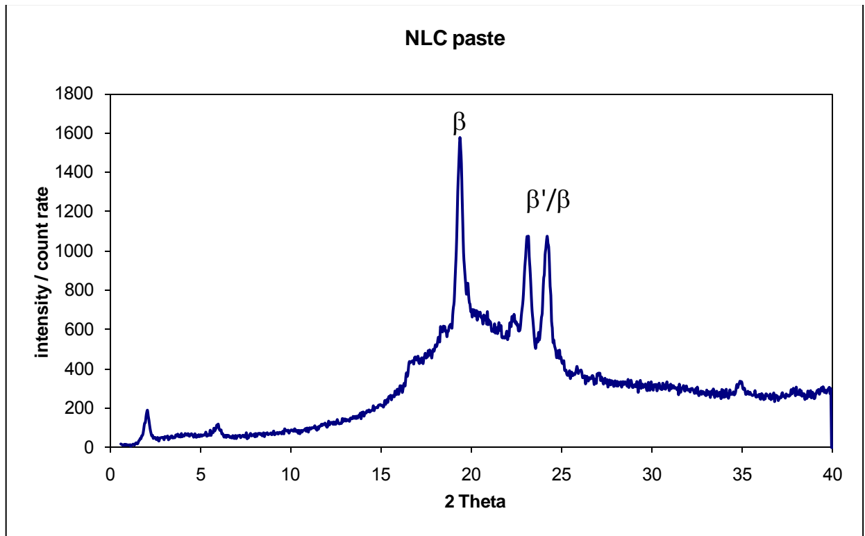
Figure 4.2.5: X-ray diffraction pattern of the NLC-paste with the \beta' and \beta modification peaks of Dynasan 118.
