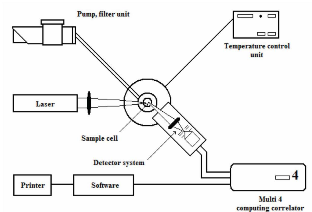
Fig. 3.2: A typical setup of a PCS apparatus. Modified after (Müller & Schuhmann, 1996).
