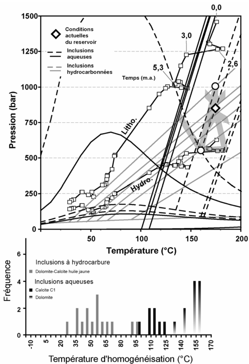
Figure 5.35. Reconstruction PVTX du puits Musgo-101.
