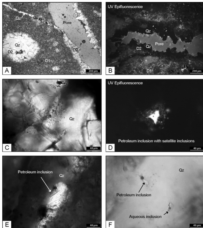
Figure 5.7. Microphotographs of samples with DPQ succession by transmitted optical microscopy (A, C, E and F) and UV-epifluorescence (B and D).
