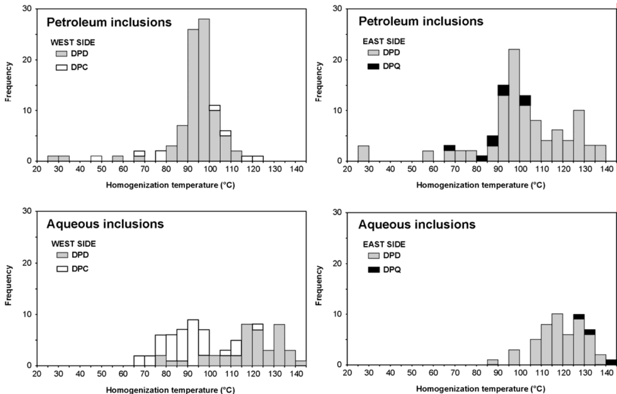
Figure 5.11. Histograms of homogenization temperatures for petroleum inclusions and aqueous inclusions from west side and east side samples.
