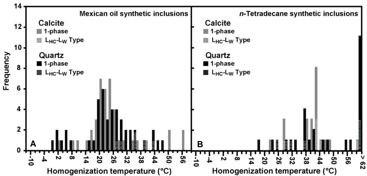
Figure 4.3. Histogram of homogenization temperatures for Mexican oil inclusions (A) and n -tetradecane inclusions (B).
