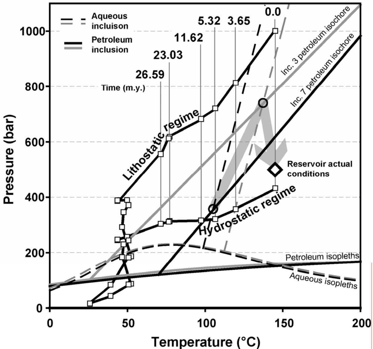
Figure 5.59. PT diagram gathering calculated isopleths and isochores after PVTX fluid inclusions analysis of both petroleum and aqueous inclusions. Crossing of contemporaneous petroleum and aqueous isochores correspond to trapping conditions. Temperature vs. hydrostatic and lithostatic gradients evolution with time calculated from well data using 1D burial modelling, are surimposed.
