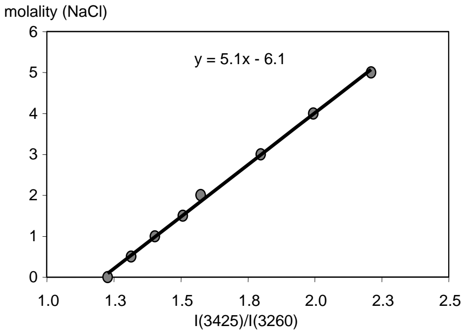
Figure 3.18. Calibration line obtained with Raman spectroscopy from standard brine ( \text{H}_2\text{O} + \text{NaCl} ) solutions at room conditions. I(3425)/I(3260) represents the intensity ratio of the Raman stretching band of water obtained with the Labram spectrometer at Nancy ( ® Horiba).
