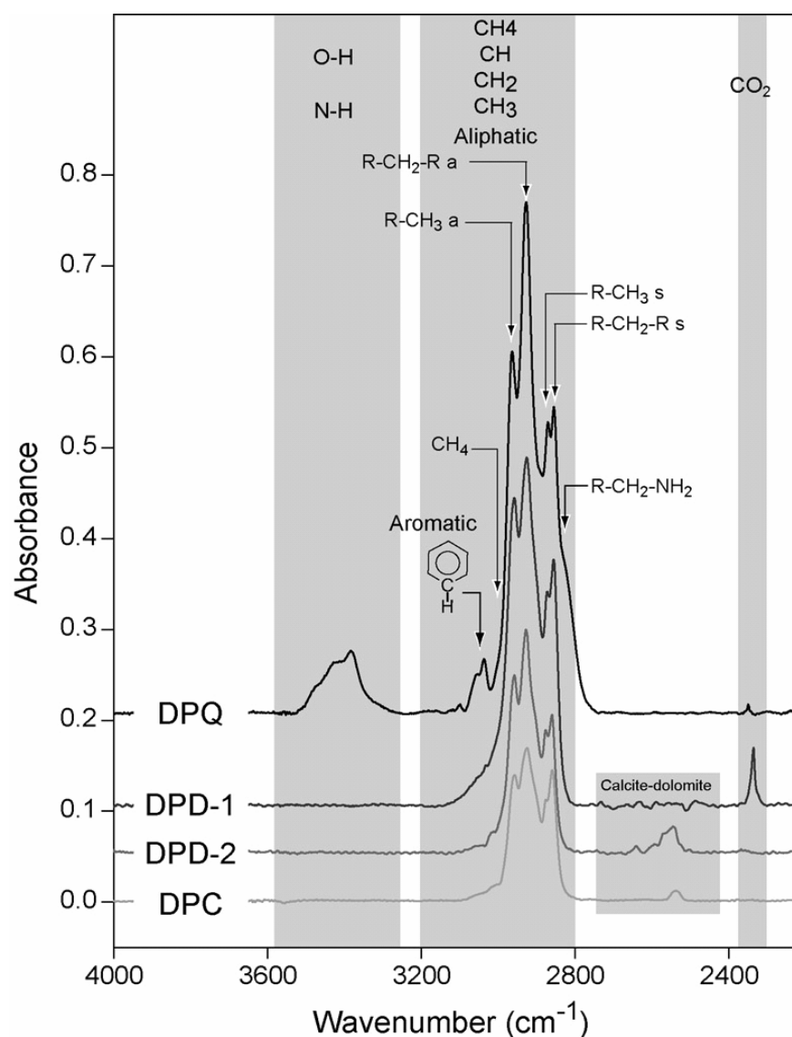
Figure 5.12. FT-IR spectra of petroleum inclusions trapped in quartz (DPQ), dolomite (DPD) or calcite (DPC) cements.
