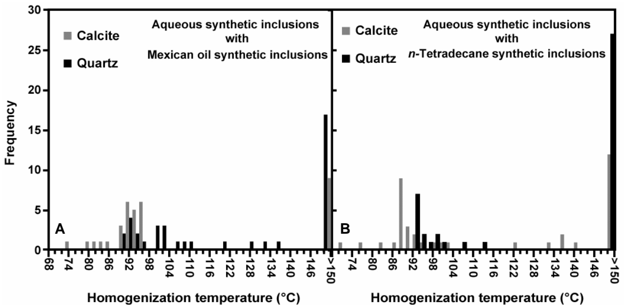
Figure 4.4. Histogram of homogenization temperatures for aqueous inclusions coeval with Mexican oil inclusions (A) and n -tetradecane inclusions (B).
