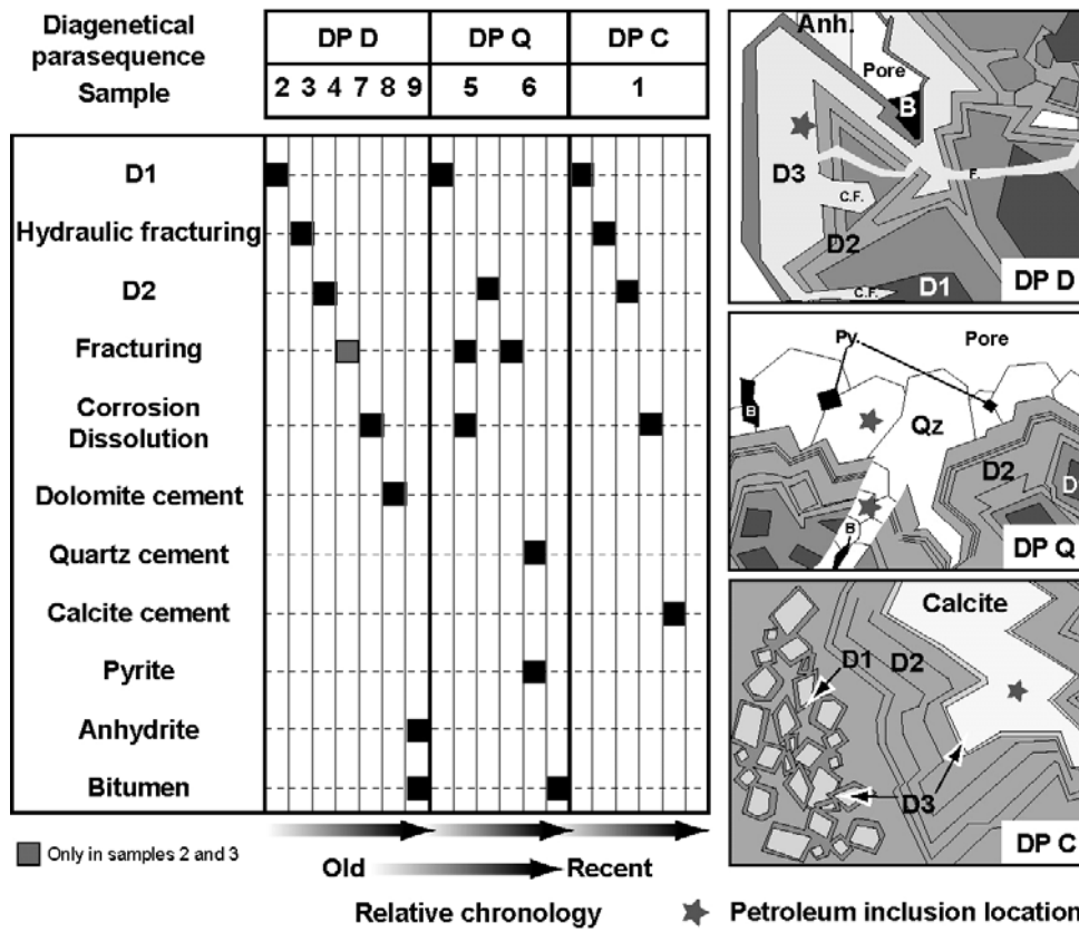
Figure 5.6. Relative chronology of diagenetical events recorded in studied samples. Py: Pyrite; B: Pyrobitumen; Qz: Quartz; Anh: anhydrite; F: Fracture; C.F.: Corrosion figure.
