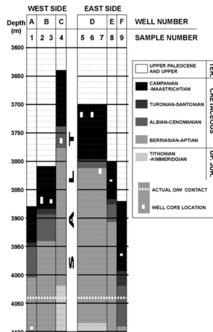
Figure 5.4. Depth location of the studied sample in the west and the east sides of the salt diapir from the Chuc oil field.
