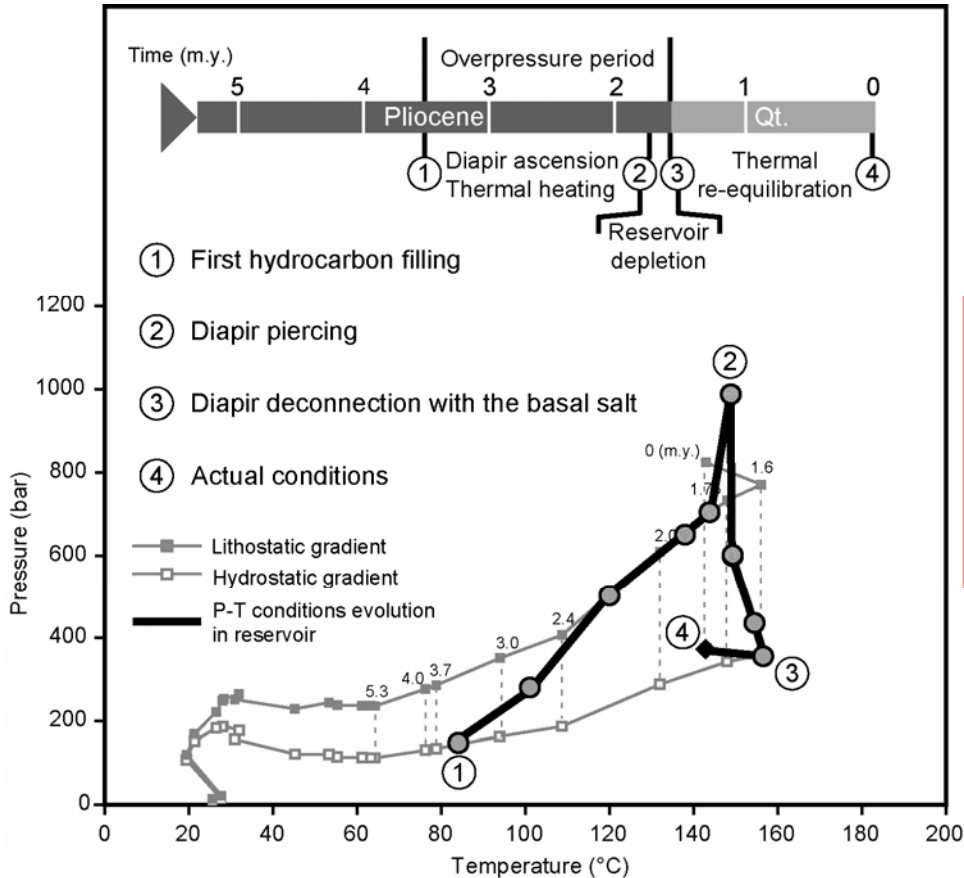
Figure 5.16. PT path for Chuc oil field with superimposition of hydrostatic and lithostatic gradients. Location of the main events of the petroleum history
