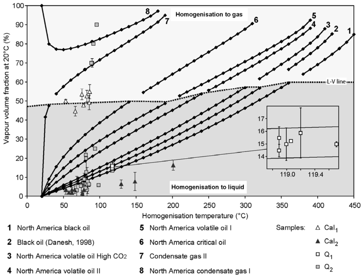
Figure 3.11. \phi_{vap} (20°C) vs. T_h for virtual inclusions having trapped eight different reference oils.
