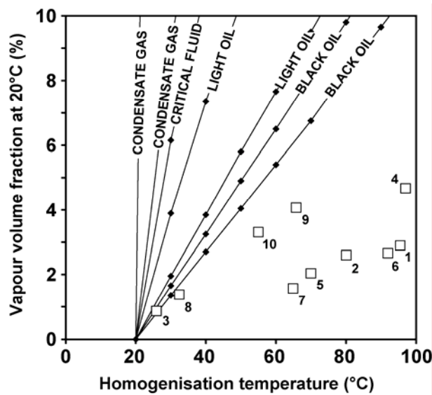
Figure 5.58. T_h vs. \phi_{vap} diagram showing CLSM and microthermometric measurements of petroleum inclusions in blocky calcite cement of Nispero field. Calibration curves with different petroleum compositions are from Bourdet et al. (submitted).
