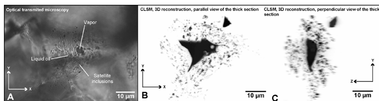
Figure 5.17. CLSM projection of a petroleum inclusion trapped in quartz showing tiny satellite inclusions. A. along x-y plane in transmission; B. along x-y plane in fluorescence; C. along z-y plane in fluorescence.
