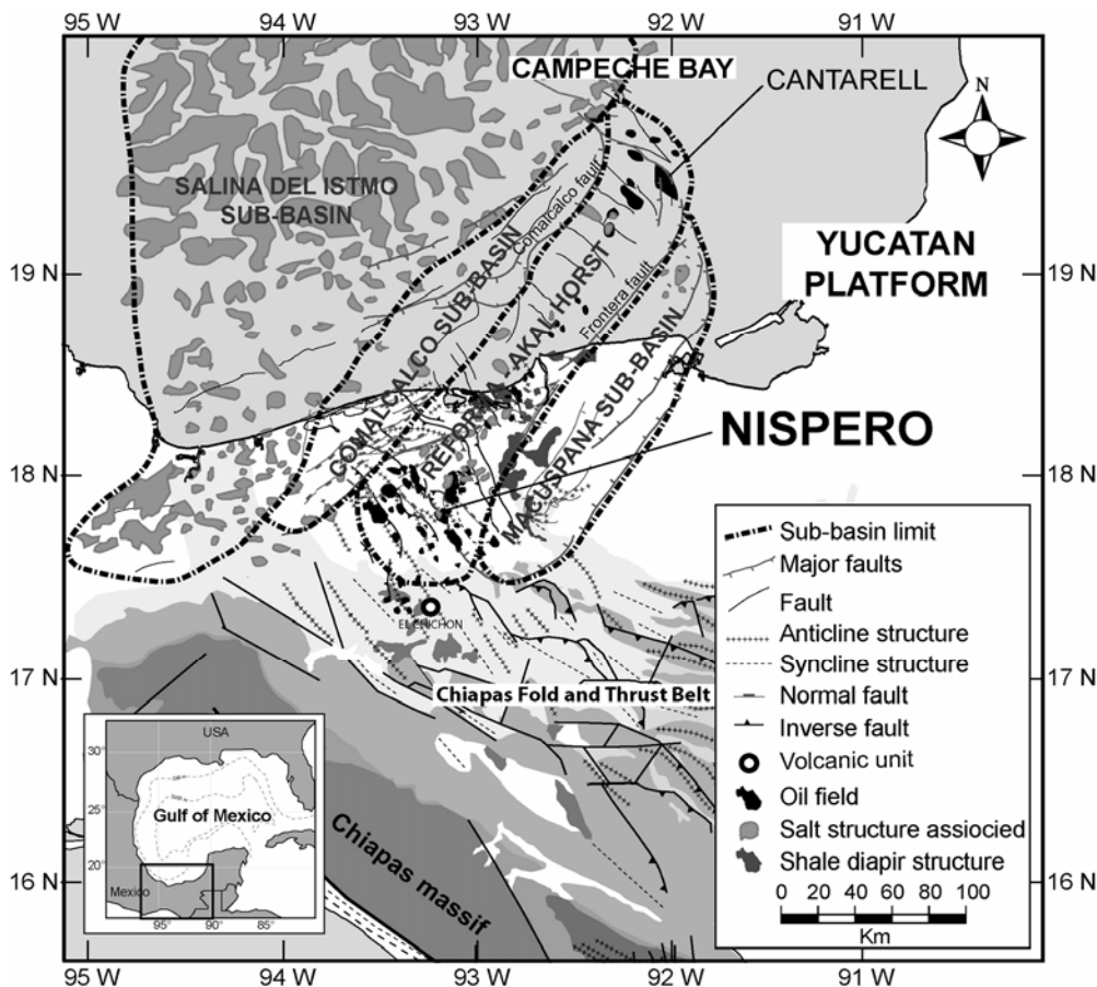
Figure 5.50. Geological setting map of Nispero field in the onshore part of the Reforma-Akal horst.
