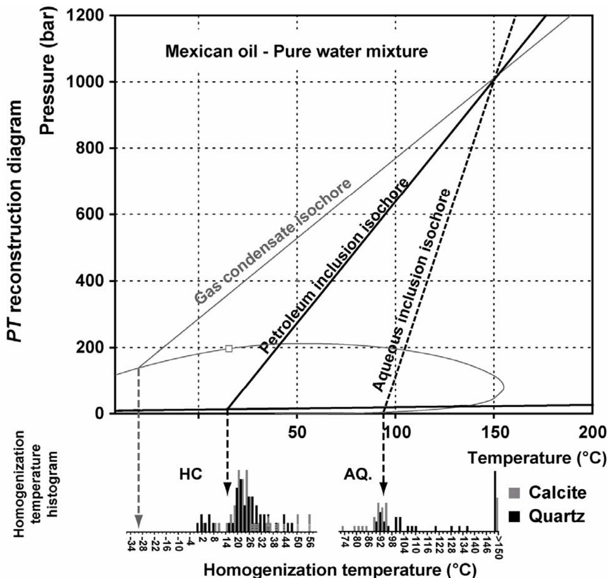
Figure 4.7. PT reconstruction diagram for Mexican oil and aqueous inclusions with corresponding measured T_h histograms. Two-phase boundary and isochore for theoretical gas condensate is reported. See figures 4.3 and 4.4 for the legend of T_h histograms.
