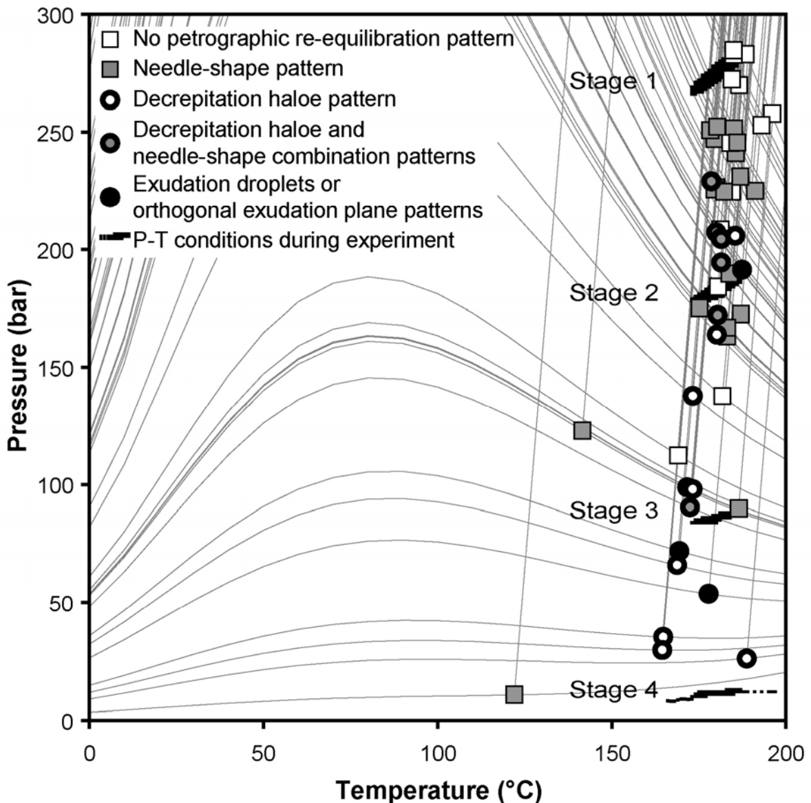
Figure 4.13. PT reconstruction diagram drawing calculated isopleths and isochores from microthermometric and Raman microspectrometric data. Each white square located at the isochore foot represent T_h and P_h conditions of each fluid inclusion measured. Small dark squares are PT conditions recorded in the autoclave during the experiment.
