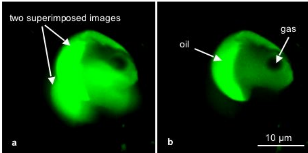
Figure 3.17. Stacks of two-dimensional images recorded by CSLM without (a) and with (b) the use of a polarizer before the collection of fluorescence by the photomultiplier.
