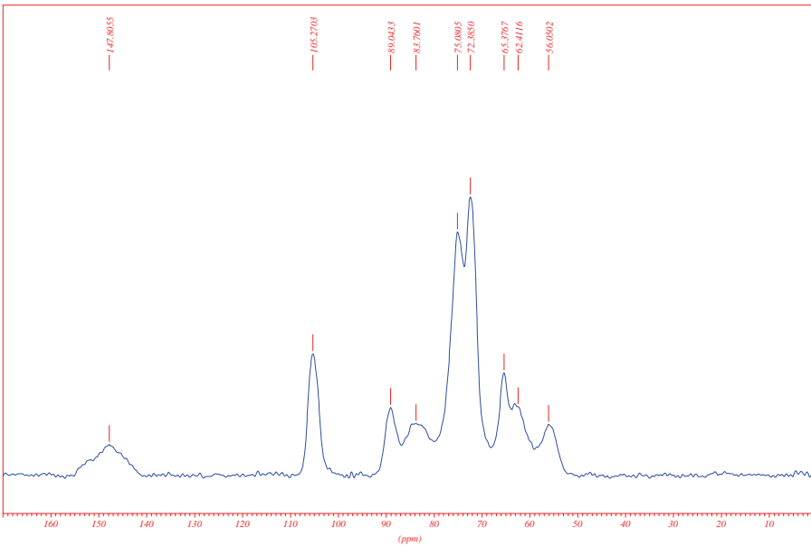
Fig. 7.2c CP-MAS 13 C-NMR spectra after G. trabeum exposure (EN 113) of heat-treated Norway spruce at high mass loss (20.5%)
