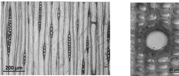
Fig. 2.6a,b Liquid full hydro-thermolysed treated Douglas fir (tangential and cross section), the parenchyma ray cells (a) and epithelial cells of resin canals (b) are not degraded and still intact
