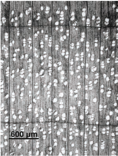
Fig. 3.4b Optimised steam hydro-thermolysis of birch (cross section), without damages of wood structure
