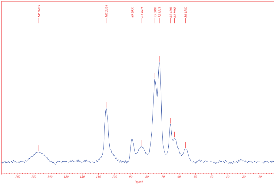
Fig. 7.2b CP-MAS ^{13}\text{C} -NMR spectra after G. trabeum exposure (EN 113) of heat-treated Norway spruce at low mass loss (0.17%)
