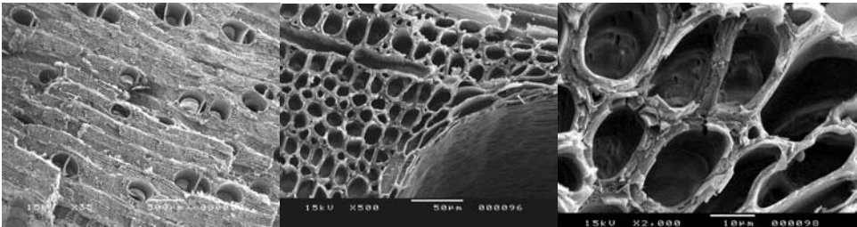
Fig. 3.8a-c Two-stage heat-treated simaruba, fracture surface after bending test
