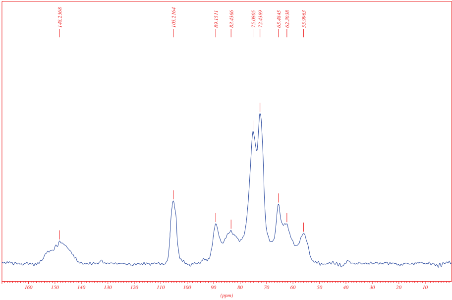
Fig. 7.3c CP-MAS 13 C-NMR spectra after P. placenta exposure (EN 113) of heat-treated Norway spruce at high mass loss (21.1%)
