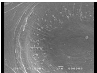
Fig. 2.10b Two-stage heat-treated Scots pine, bordered pit with opened pit chamber
