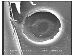
Fig. 2.11b Two-stage heat-treated Spruce, bordered pit with opened pit chamber
