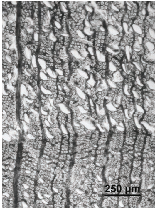
Fig. 3.1a Hydro-thermolysed treated beech (cross section), serious collapse of vessels
