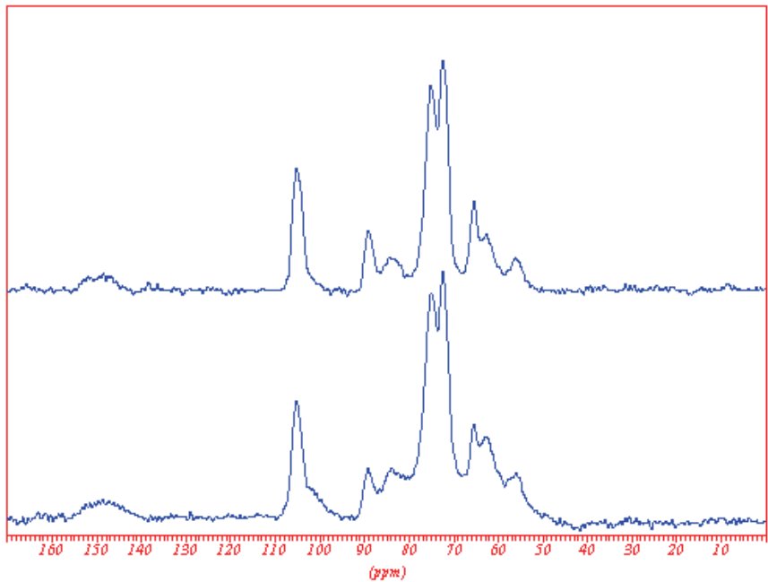
Fig. 8.2 CP MAS 13 CNMR spectra after fungal exposure in ground contact (EN 252) of untreated (below) and heat-treated (above) radiata pine
