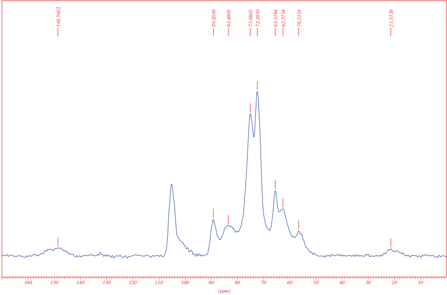
Fig. 7.4a CP-MAS 13 C-NMR spectra after C. versicolor exposure (EN 113) of untreated Scots pine sapwood (mass loss 27.8%)
