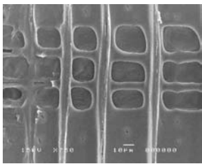
Fig. 2.10c Two-stage heat-treated Scots pine, radial section, crossing field
