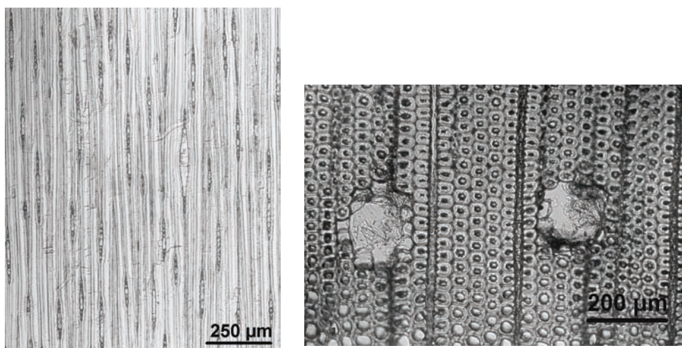
Fig. 2.5a,b Liquid full hydro-thermolysed treated Scots pine (tangential and cross section), damaged parenchyma ray cells (a) and epithelial cells of resin canals (b). The ray tracheids are still intact
