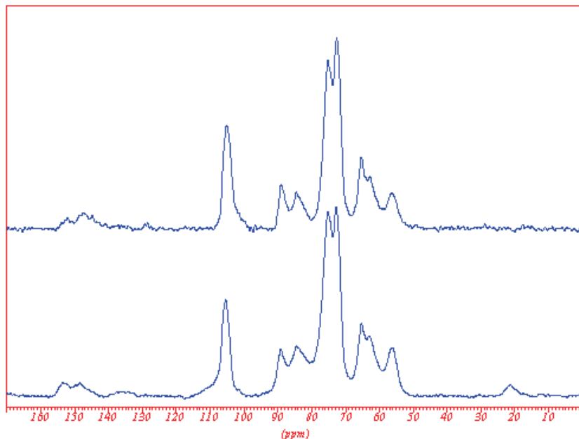
Fig. 8.5 CP MAS ^{13}\text{C} NMR spectra after fungal exposure in ground contact (EN 252) of untreated (below) and heat-treated (above) simaruba
