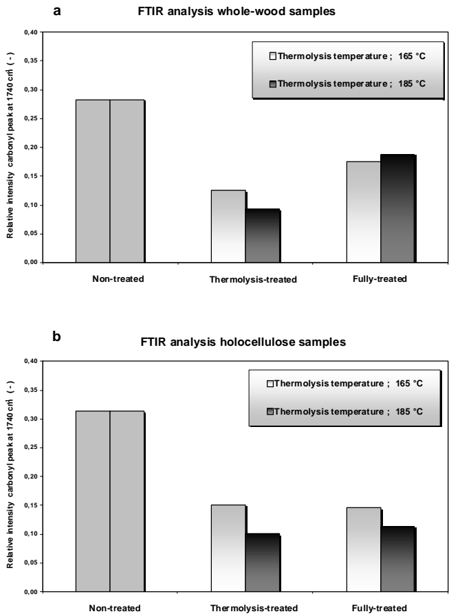
Fig. 4a and b Relative intensity of carbonyl peak in the FTIR spectra of heat-treated Scots Pine at different temperatures; (a) pine wood; (b) holocellulose
