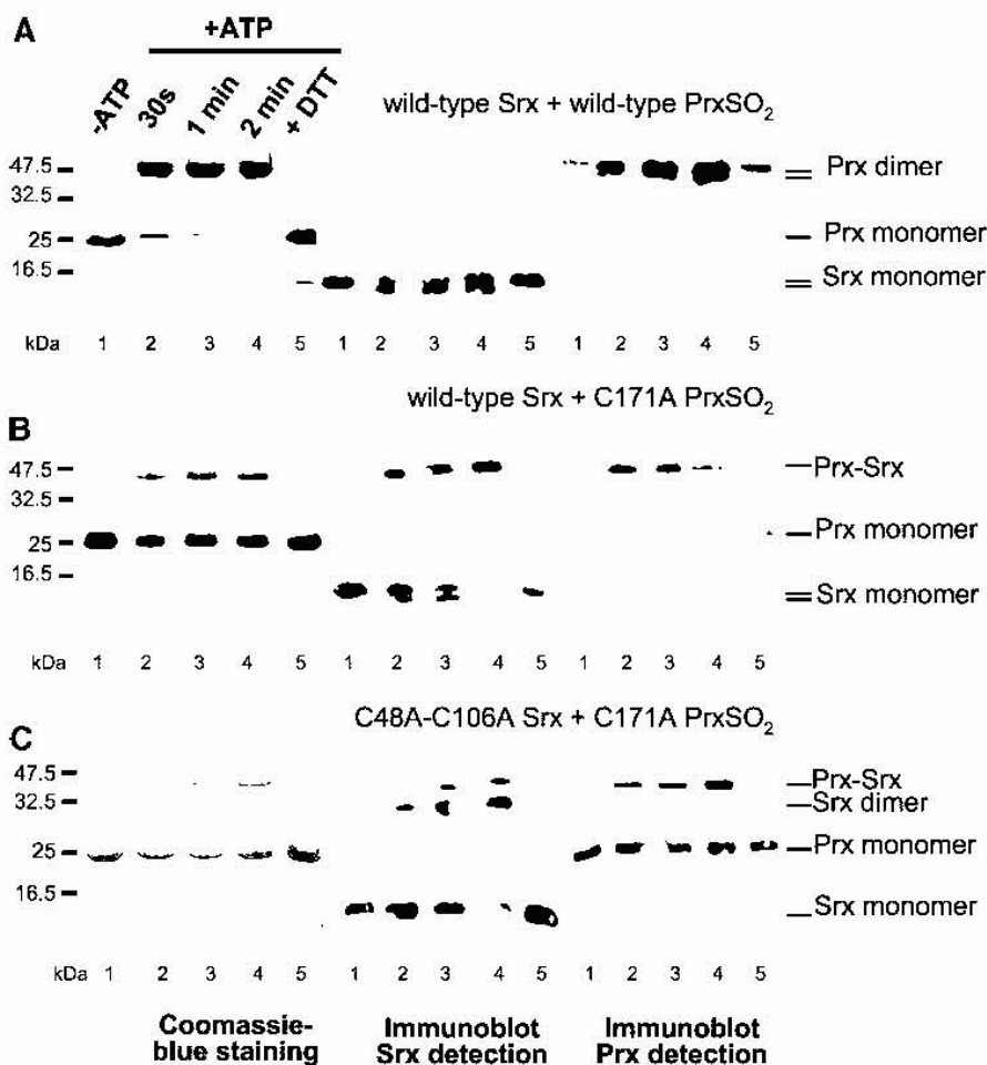
FIGURE 2. Non-reducing SDS-PAGE and immunoblot analysis of the species formed for the reaction catalyzed by Srx in the absence of added reducer. Equimolar concentrations (30 \mu M) of Srx and PrxSO 2 were mixed in the absence (lane 1) or presence of 1 mM ATP-MgCl 2 for the indicated times (lanes 2–4), and for 2 min followed by the addition of 50 mM DTT (lane 5), immediately followed by addition of 25 mM IAM and non-reducing SDS-PAGE fractionation. Reactions were carried out in TK buffer at 30°C. Three identical SDS-PAGE gels were run in parallel for Coomassie Blue staining (left panel) or immunoblot revelation against Srx (middle panel) and His tag (right panel) specific antisera. A, wild-type PrxSO 2 and wild-type Srx; bands corresponding to monomeric Prx in the immunoblot are very faint due to the relative amounts and sensitivity to His tag antisera of both species; B, C171A PrxSO 2 and wild-type Srx; C, C171A PrxSO 2 and C48A-C106A Srx.
