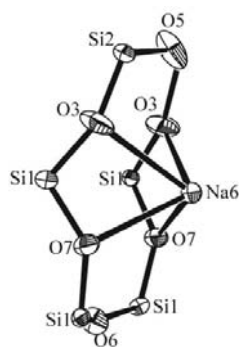
Figure 4.7 : Coordination de Na6
