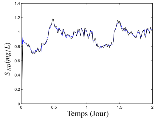
(b) La concentration S_{ND}(mg/L)
