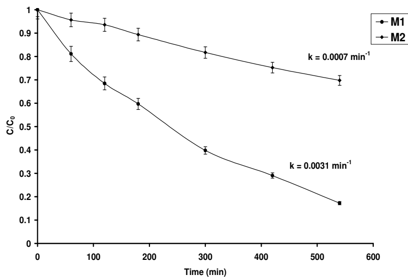
Figure 4.8. H 2 O 2 decomposition at 1g/L of both solids (M1, and M2). [H 2 O 2 ] = 1 mM, 20°C, pH7.
