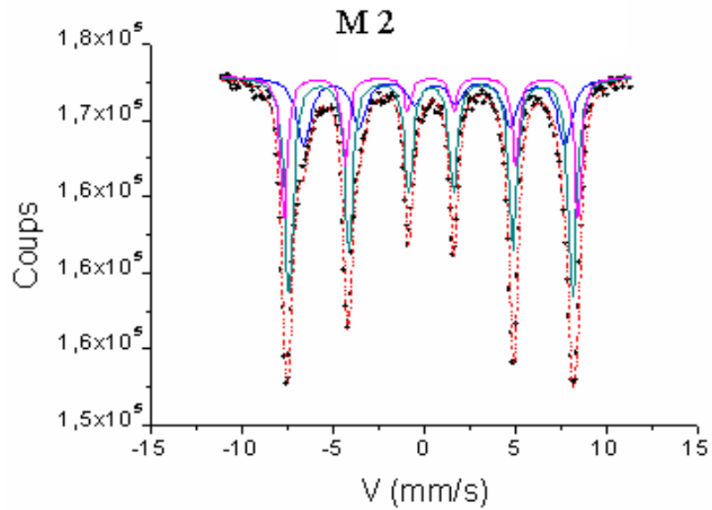
Figure 4.2. Mössbauer spectra data about two kinds of iron oxides used in this work (M1 and M2).
