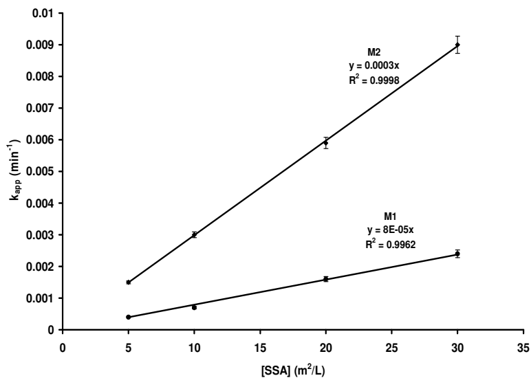
Figure 4.9. H 2 O 2 decomposition rate versus [SSA]. [H 2 O 2 ] = 1 mM, 20°C, pH7.
