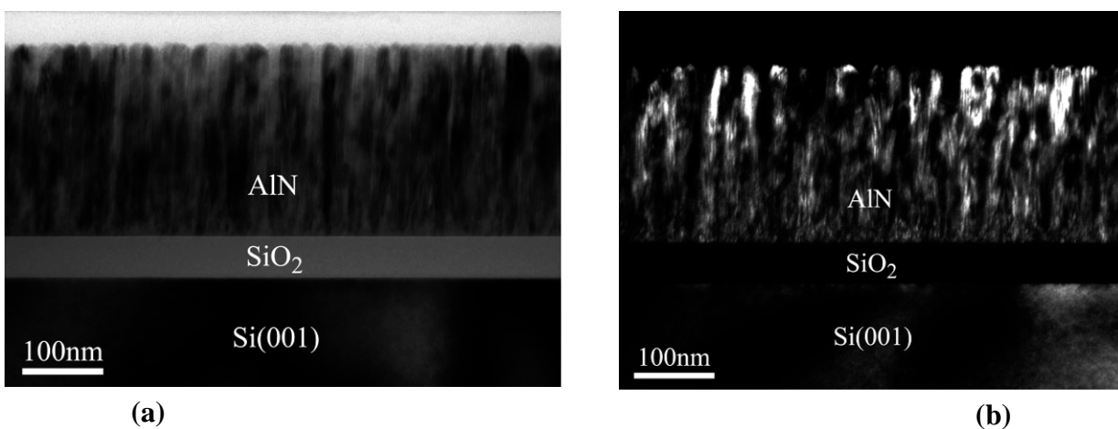
Figure 5.4 : (a) Champ clair ; (b) Champ sombre
