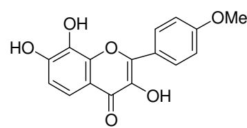
Retusin
