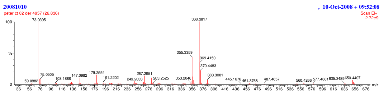
(+)-catechin, rt = 26.83 min
