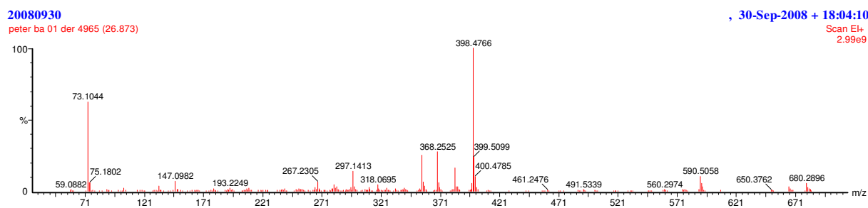
bark main component, rt = 26.87 min.
